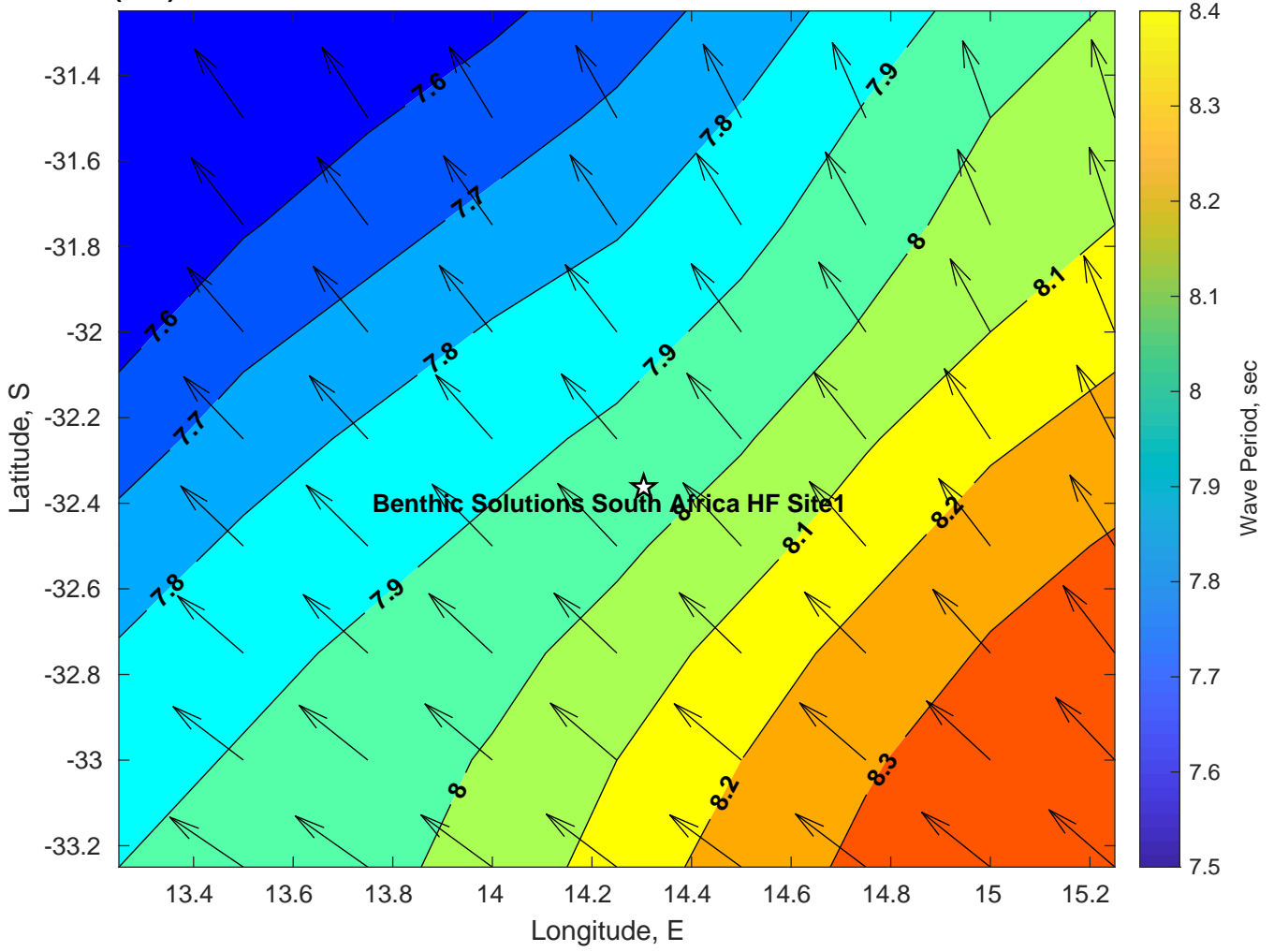
Wave Period (sec) for Benthic Solutions South Africa HF Site1 at 28-Mar-2025 09:00:00
