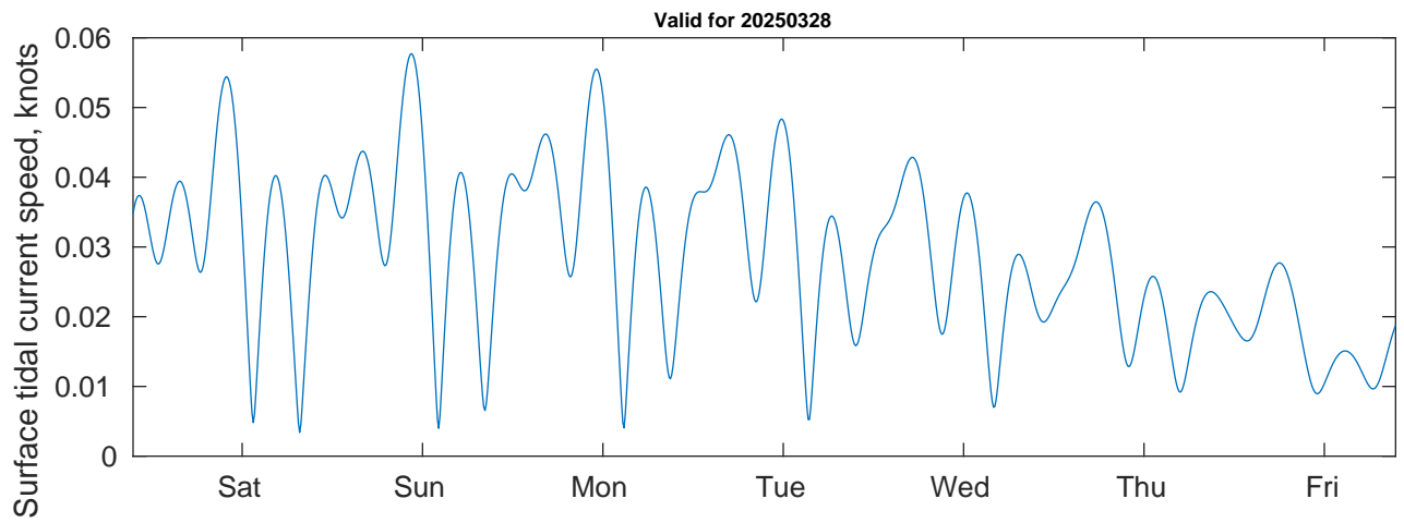
Tidal Currents and Heights for Benthic Solutions South Africa HF Site1 at 20250328
