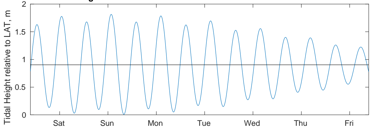
Tidal Currents and Heights for Benthic Solutions South Africa HF Site1 at 20250328
