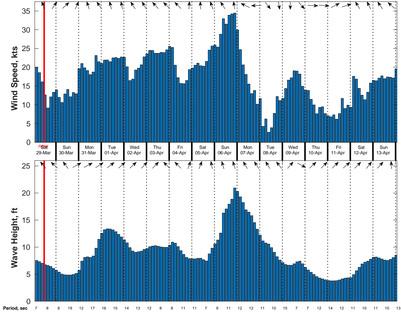
Wind & Wave Forecast for Benthic Solutions South Africa HF Site1 from 28-Mar-2025 02:00:00 to 13-Apr-2025 02:00:00
