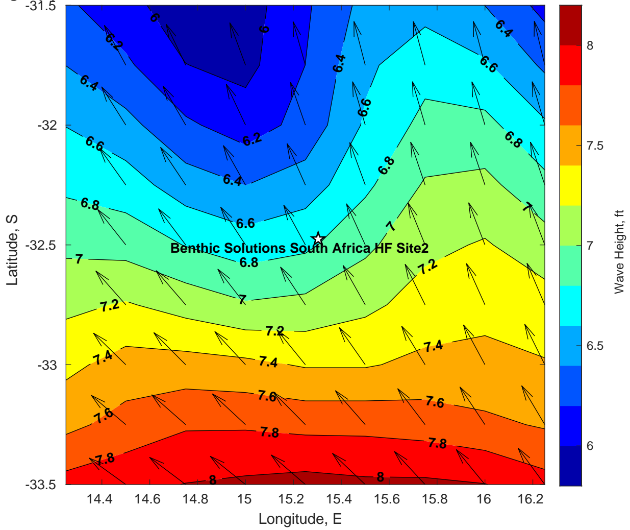
Wave Height (ft) for Benthic Solutions South Africa HF Site2 at 28-Mar-2025 09:00:00
