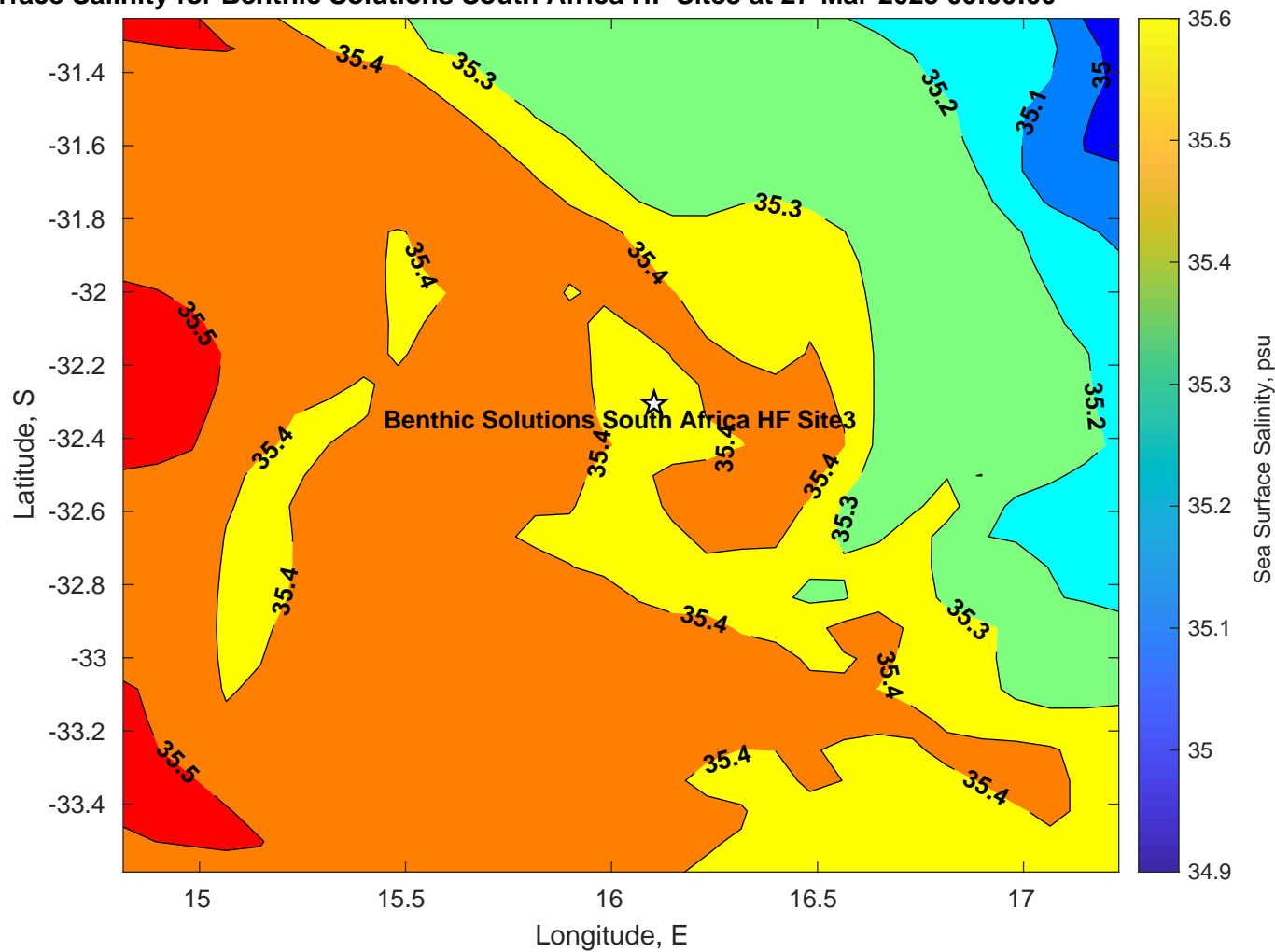
Surface Salinity for Benthic Solutions South Africa HF Site3 at 27-Mar-2025 00:00:00
