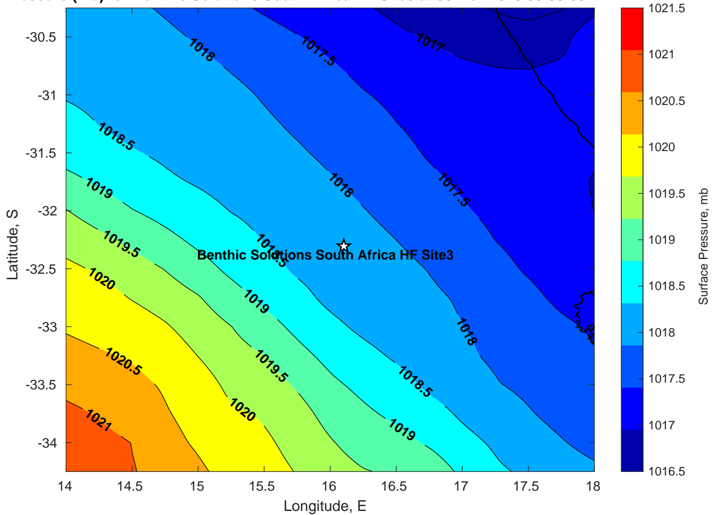
Surface Pressure (mb) for Benthic Solutions South Africa HF Site3 at 30-Mar-2025 00:00:00
