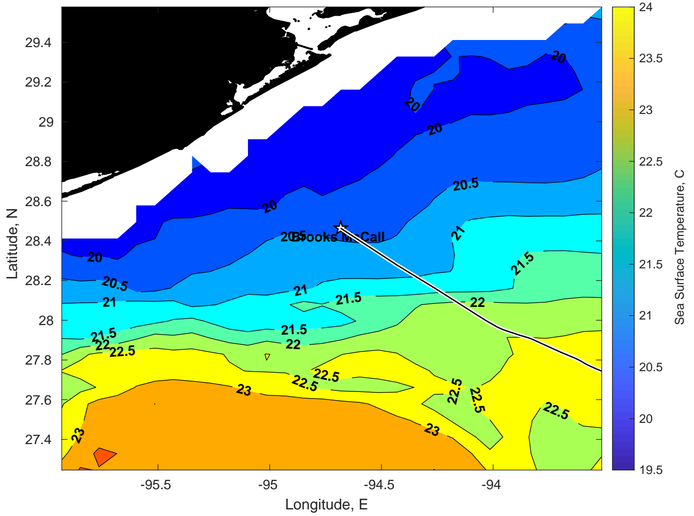
SST for Brooks McCall at 27-Mar-2025 00:00:00
