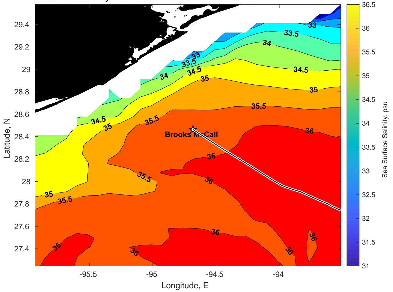
Surface Salinity for Brooks McCall at 27-Mar-2025 00:00:00
