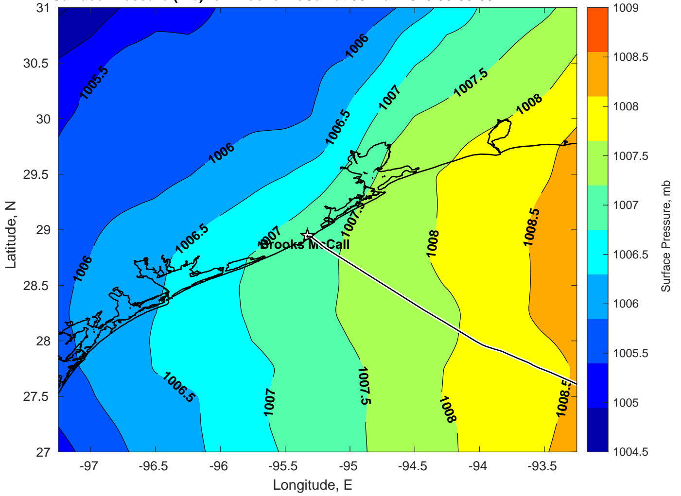
Surface Pressure (mb) for Brooks McCall at 30-Mar-2025 00:00:00
