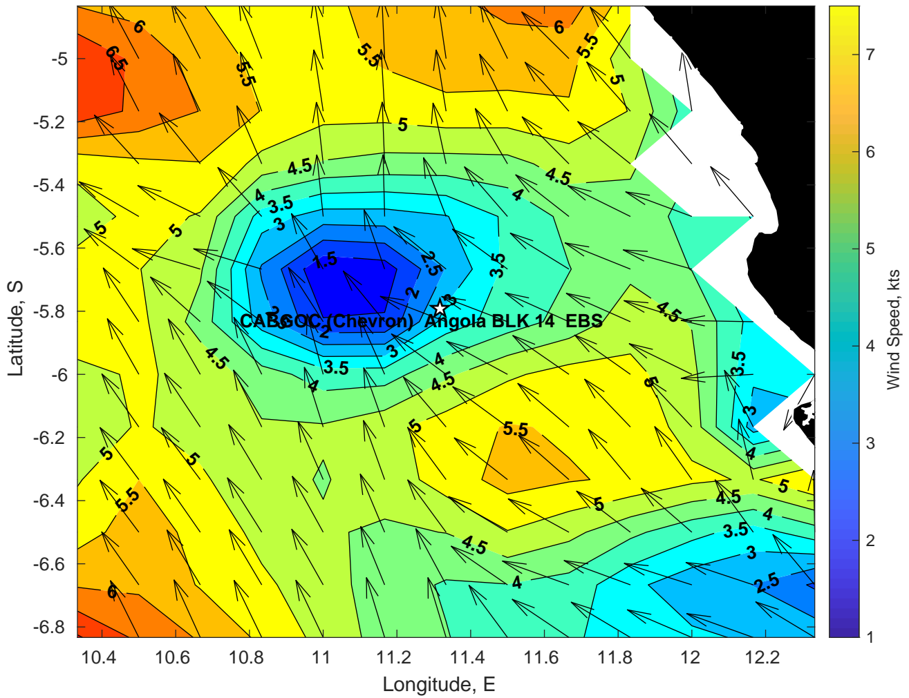
Winds (kts) for CABGOC (Chevron) Angola BLK 14 EBS at 28-Mar-2025 09:00:00
