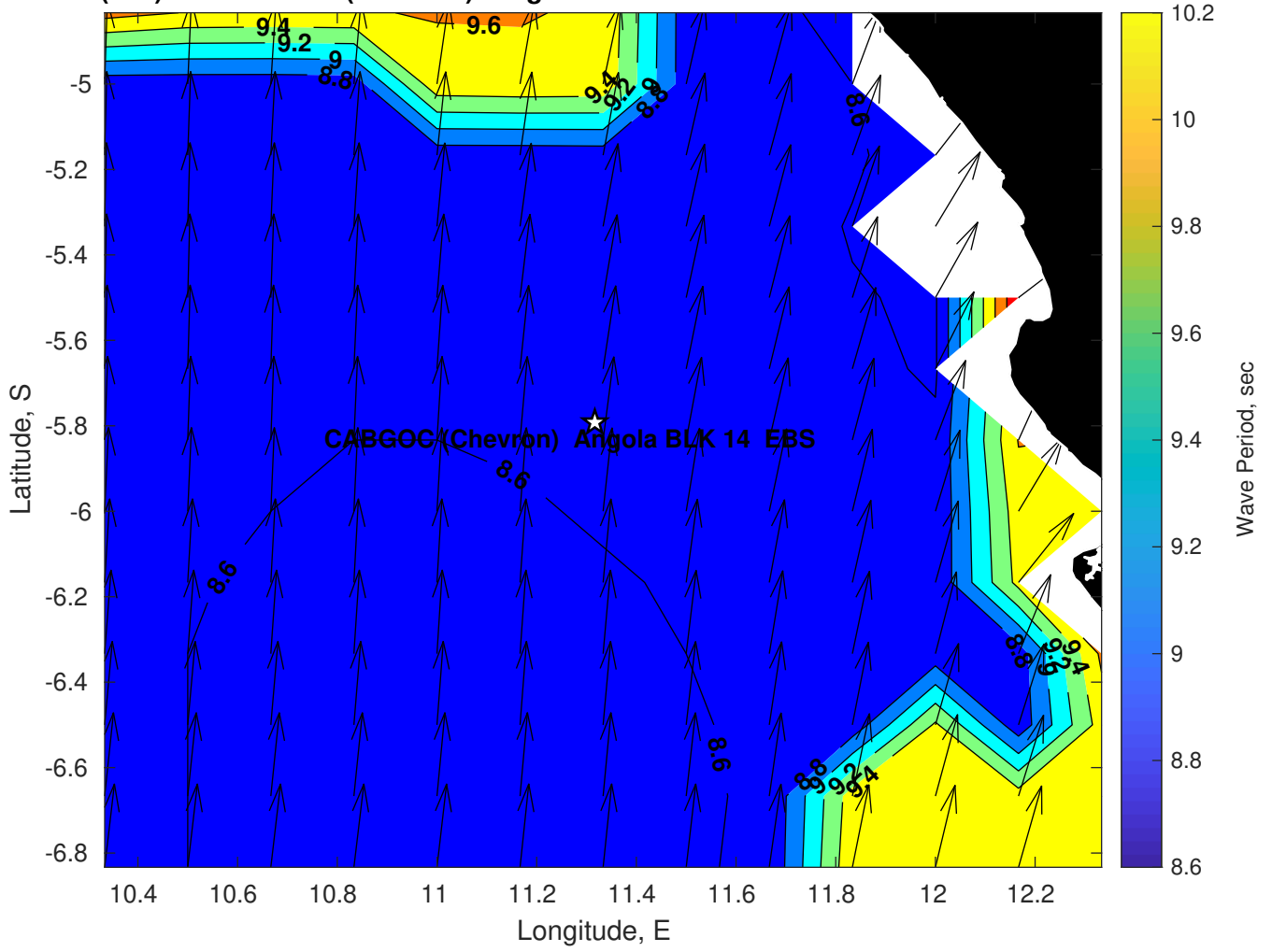
Wave Period (sec) for CABGOC (Chevron) Angola BLK 14 EBS at 28-Mar-2025 09:00:00
