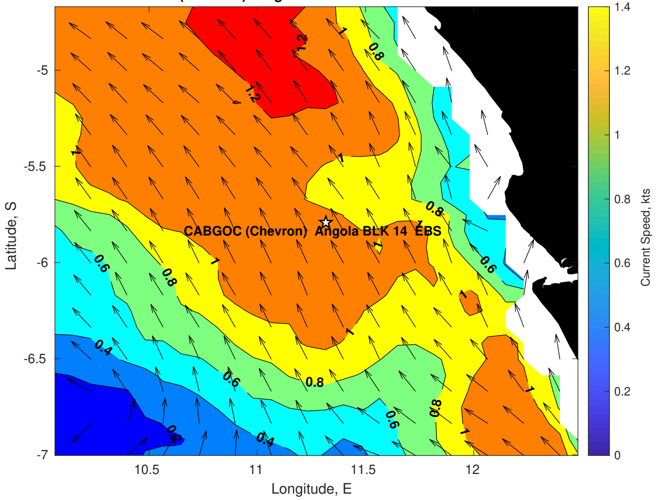
Surface Currents for CABGOC (Chevron) Angola BLK 14 EBS at 27-Mar-2025 00:00:00
