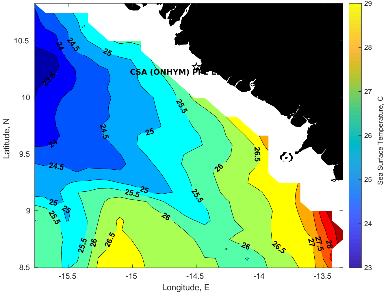
SST for CSA (ONHYM) PPL EBS - Guinea at 27-Mar-2025 00:00:00
