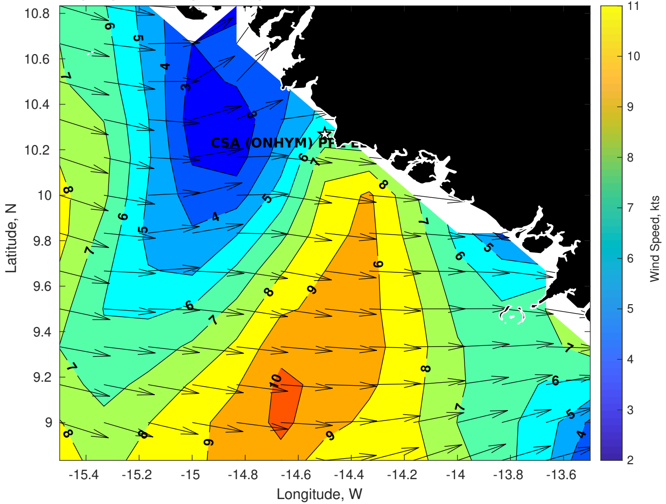
Winds (kts) for CSA (ONHYM) PPL EBS - Guinea at 28-Mar-2025 09:00:00
