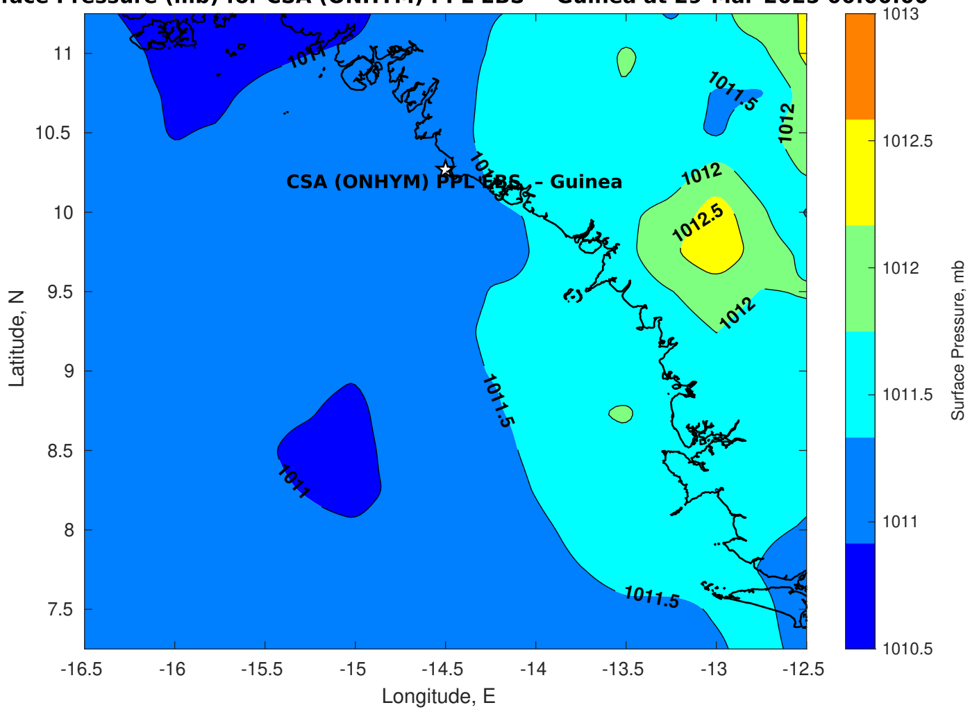
Surface Pressure (mb) for CSA (ONHYM) PPL EBS - Guinea at 29-Mar-2025 00:00:00
