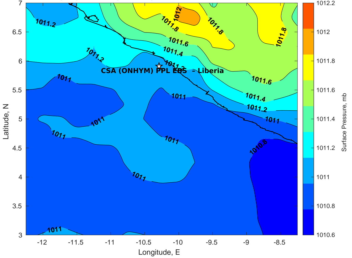
Surface Pressure (mb) for CSA (ONHYM) PPL EBS - Liberia at 29-Mar-2025 00:00:00
