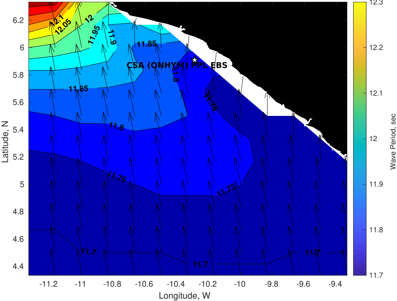
Wave Period (sec) for CSA (ONHYM) PPL EBS - Liberia at 28-Mar-2025 09:00:00
