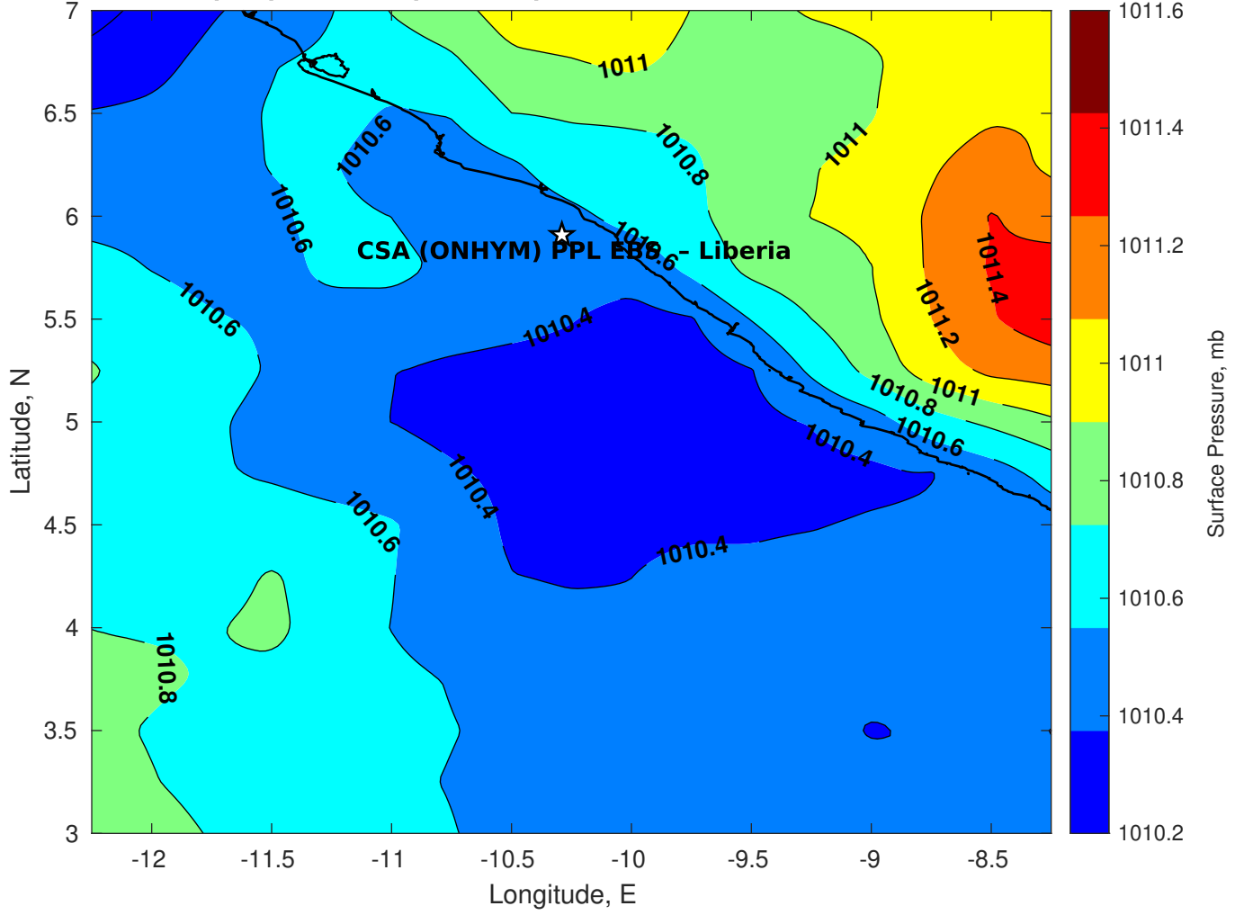
Surface Pressure (mb) for CSA (ONHYM) PPL EBS - Liberia at 30-Mar-2025 00:00:00
