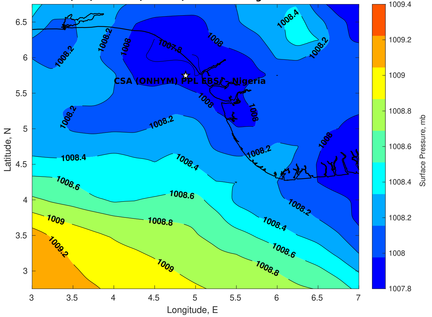
Surface Pressure (mb) for CSA (ONHYM) PPL EBS - Nigeria at 29-Mar-2025 00:00:00
