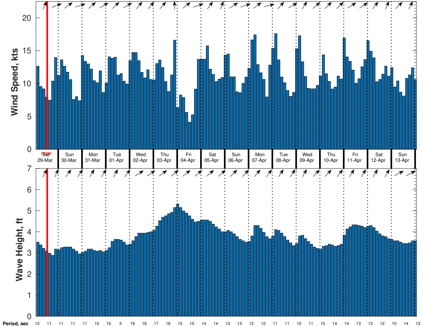
Wind & Wave Forecast for CSA (ONHYM) PPL EBS - Nigeria from 28-Mar-2025 02:00:00 to 13-Apr-2025 02:00:00
