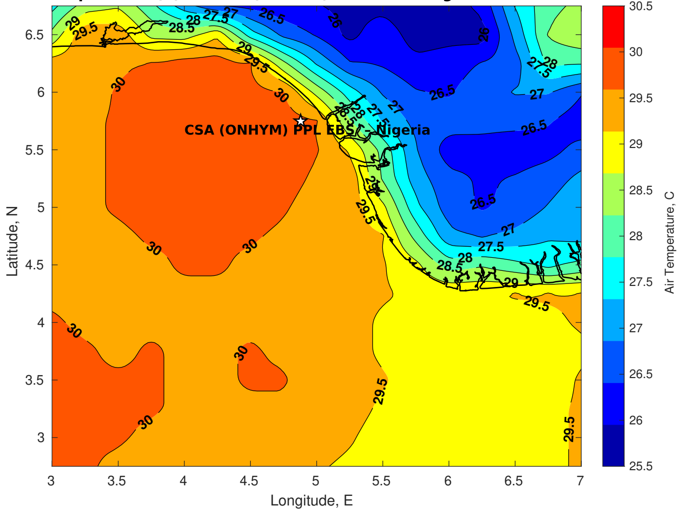
Air Temperature (C) for CSA (ONHYM) PPL EBS - Nigeria at 28-Mar-2025
