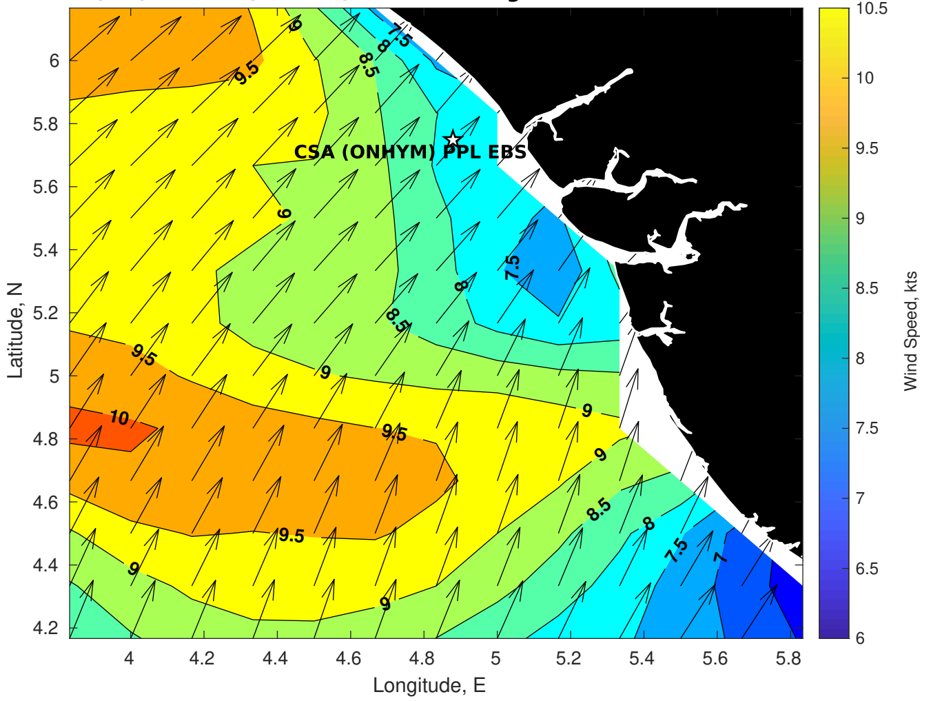
Winds (kts) for CSA (ONHYM) PPL EBS - Nigeria at 28-Mar-2025 09:00:00
