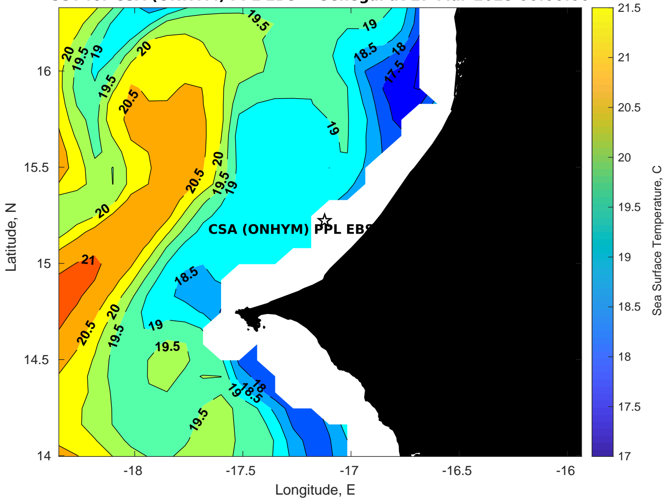
SST for CSA (ONHYM) PPL EBS - Senegal at 27-Mar-2025 00:00:00
