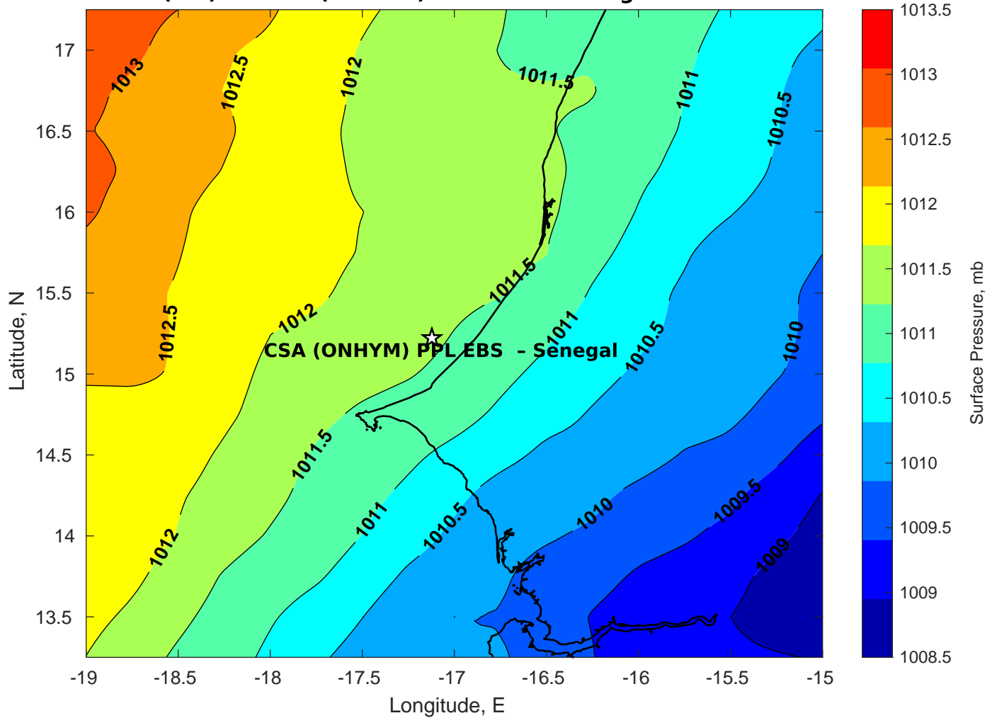
Surface Pressure (mb) for CSA (ONHYM) PPL EBS - Senegal at 28-Mar-2025 00:00:00
