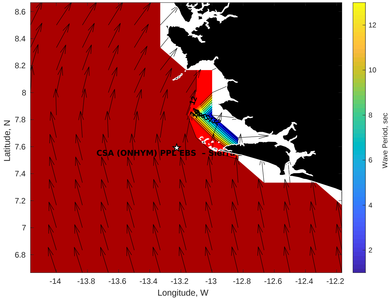
Wave Period (sec) for CSA (ONHYM) PPL EBS - Sierra Leone at 28-Mar-2025 09:00:00
