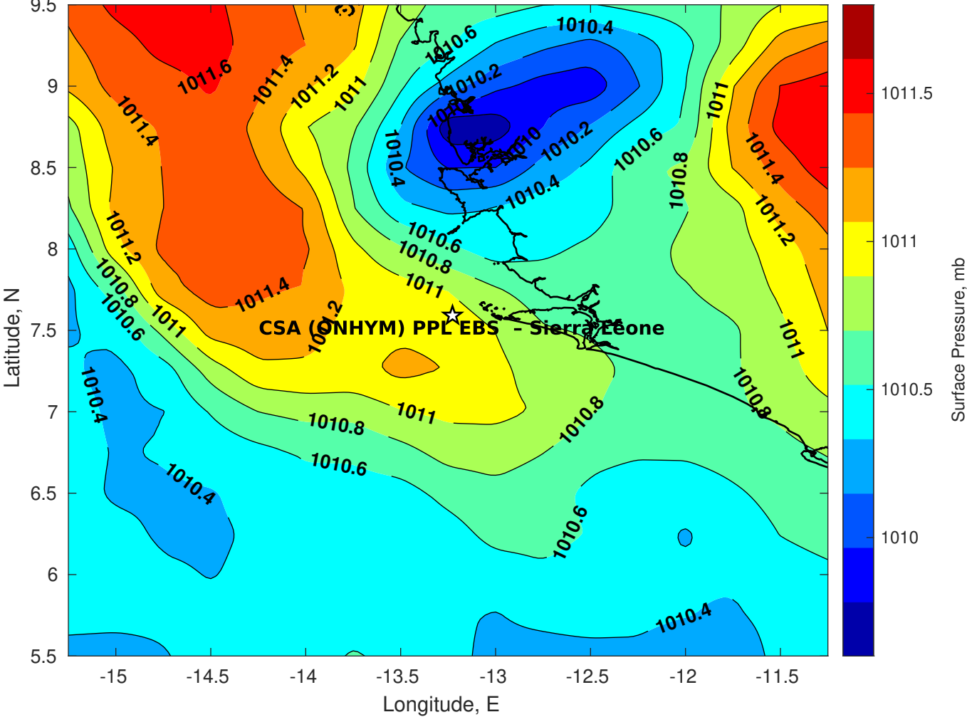
Surface Pressure (mb) for CSA (ONHYM) PPL EBS - Sierra Leone at 28-Mar-2025 00:00:00
