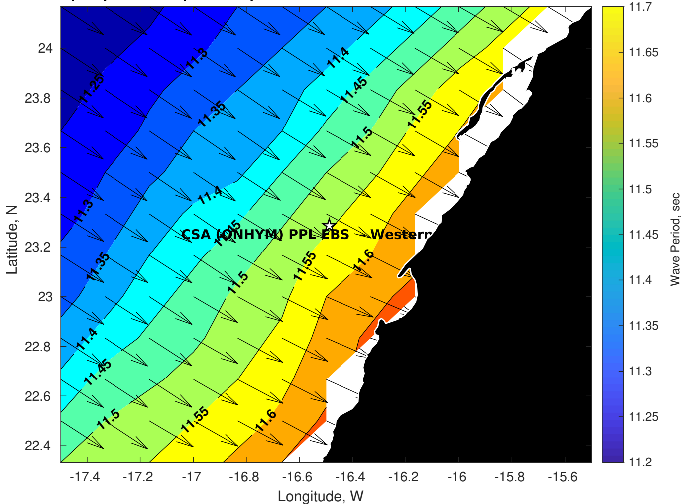
Wave Period (sec) for CSA (ONHYM) PPL EBS - Western Sahara at 28-Mar-2025 09:00:00
