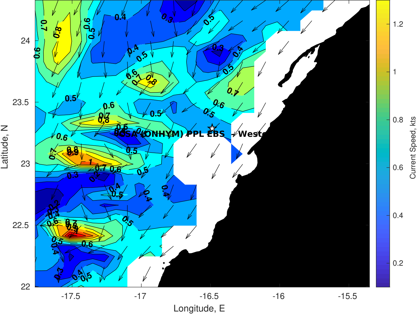
Surface Currents for CSA (ONHYM) PPL EBS - Western Sahara at 27-Mar-2025 00:00:00
