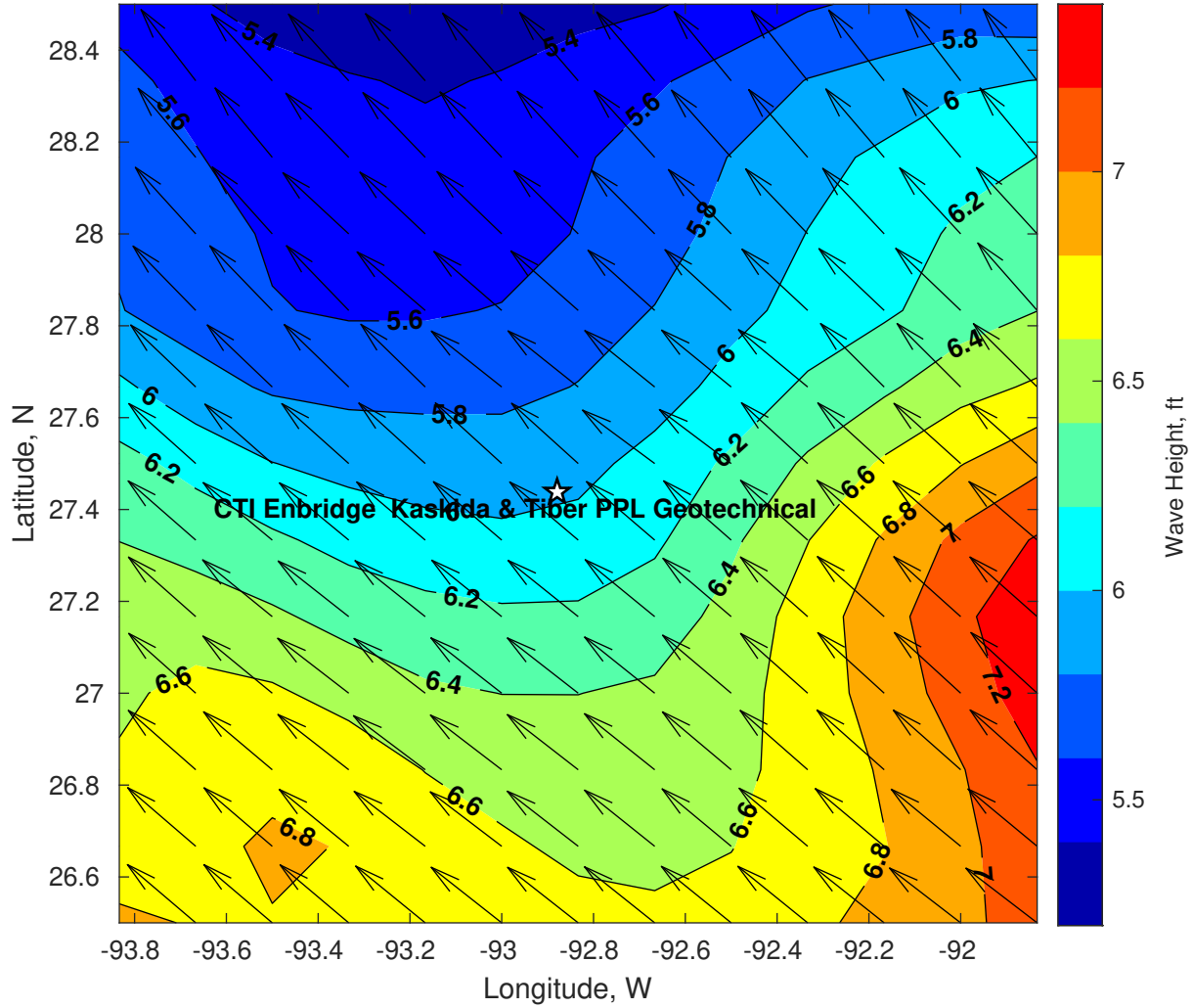
Wave Height (ft) for CTI Enbridge Kaskida & Tiber PPL Geotechnical at 28-Mar-2025 09:00:00
