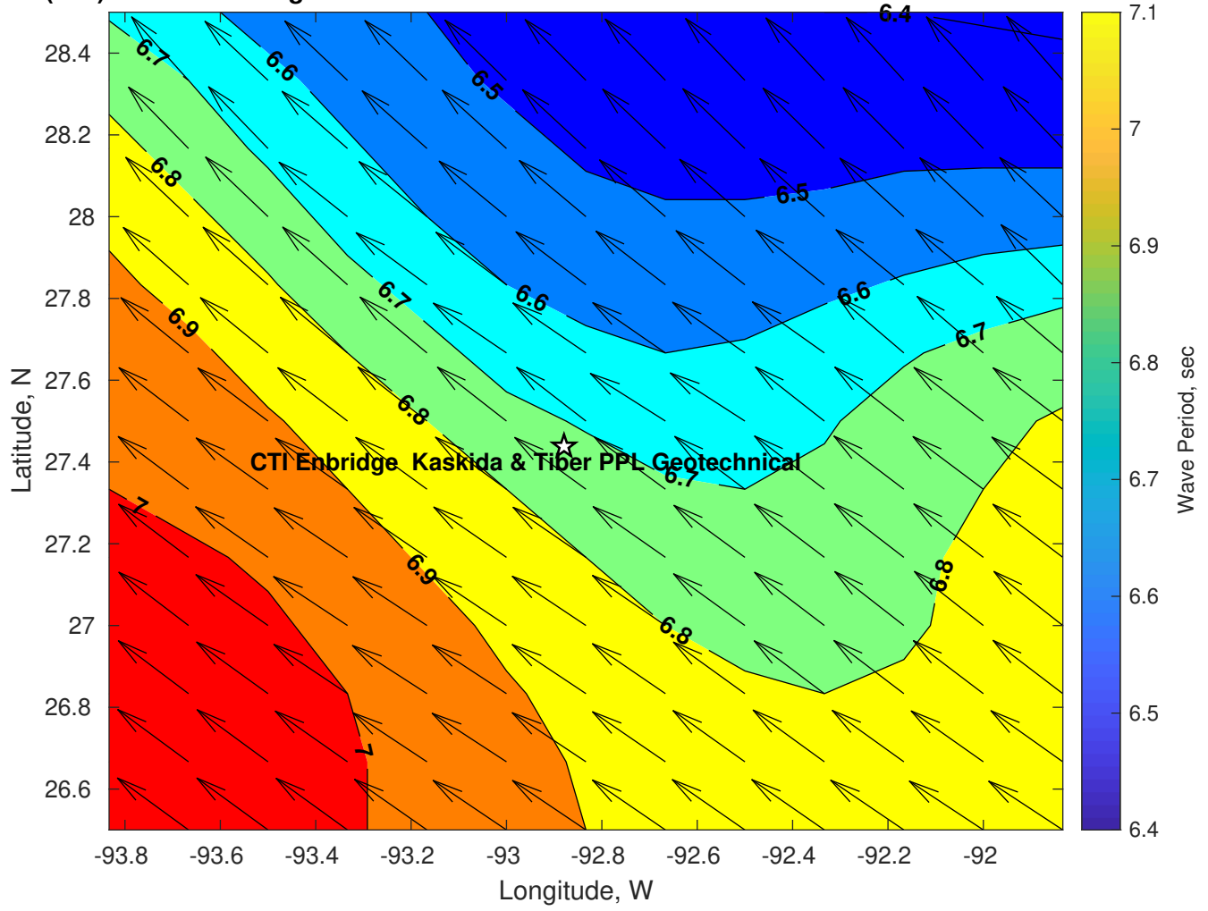
Wave Period (sec) for CTI Enbridge Kaskida & Tiber PPL Geotechnical at 28-Mar-2025 09:00:00
