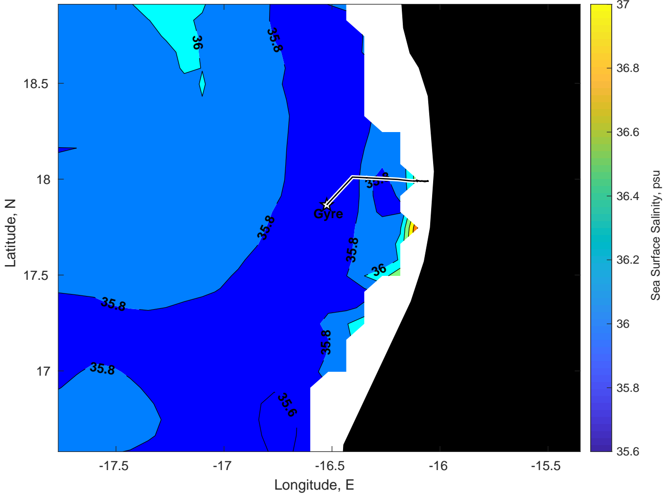
Surface Salinity for Gyre at 27-Mar-2025 00:00:00
