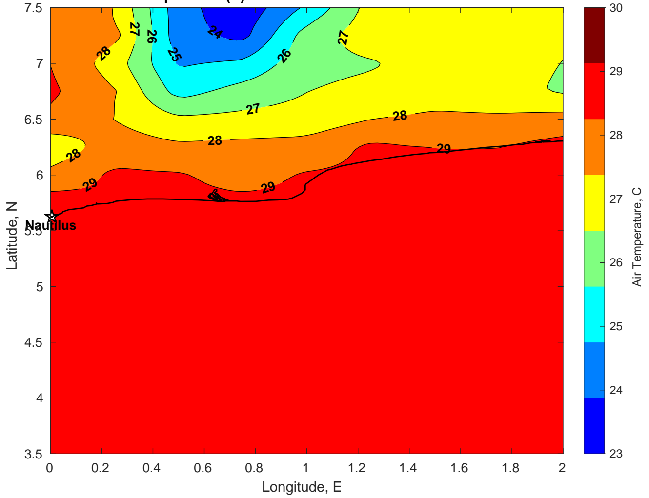
Air Temperature (C) for Nautilus at 28-Mar-2025
