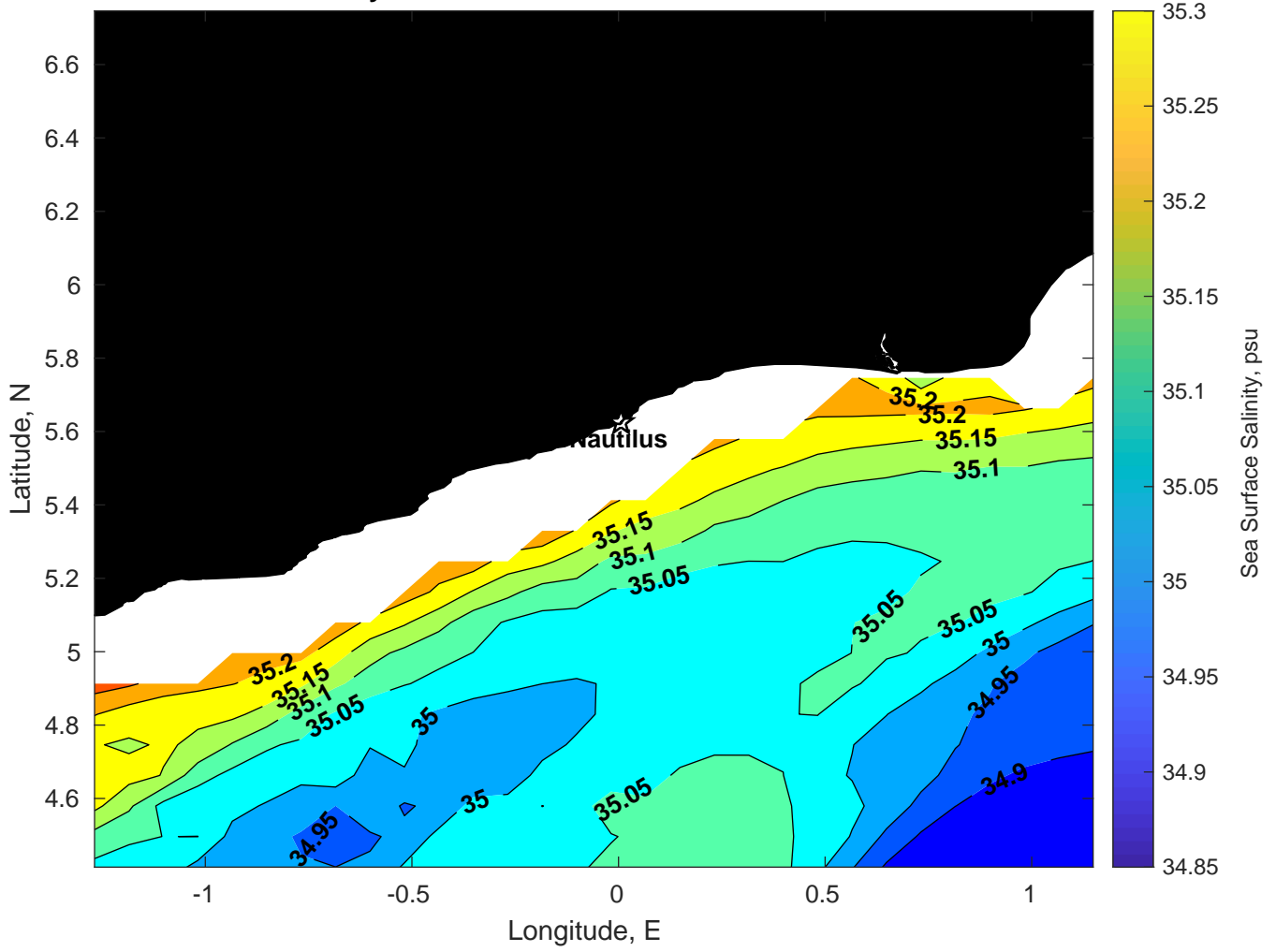
Surface Salinity for Nautilus at 27-Mar-2025 00:00:00
