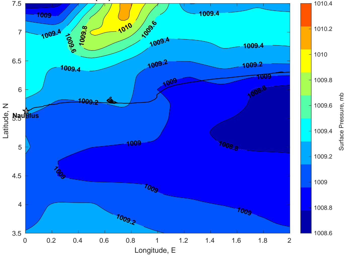
Surface Pressure (mb) for Nautilus at 28-Mar-2025 00:00:00
