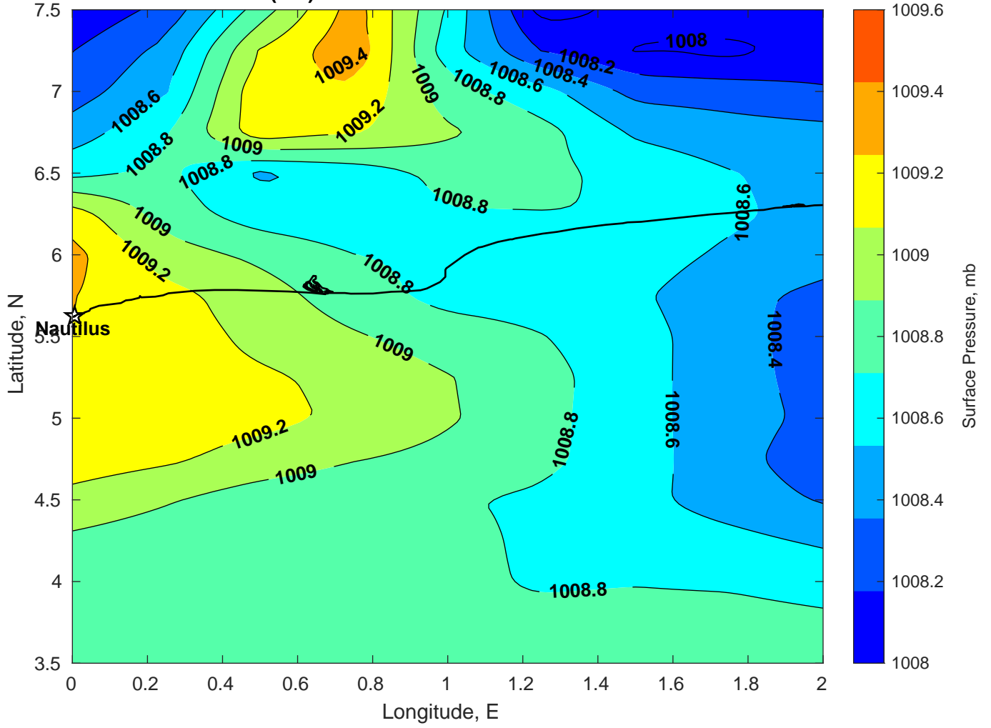
Surface Pressure (mb) for Nautilus at 30-Mar-2025 00:00:00
