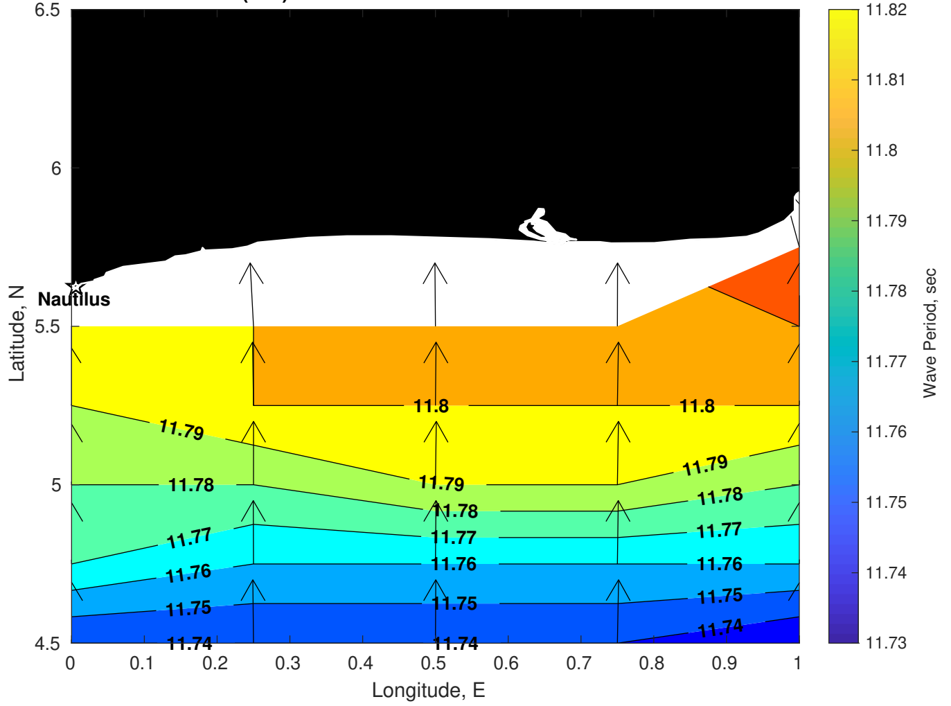
Wave Period (sec) for Nautilus at 28-Mar-2025 09:00:00
