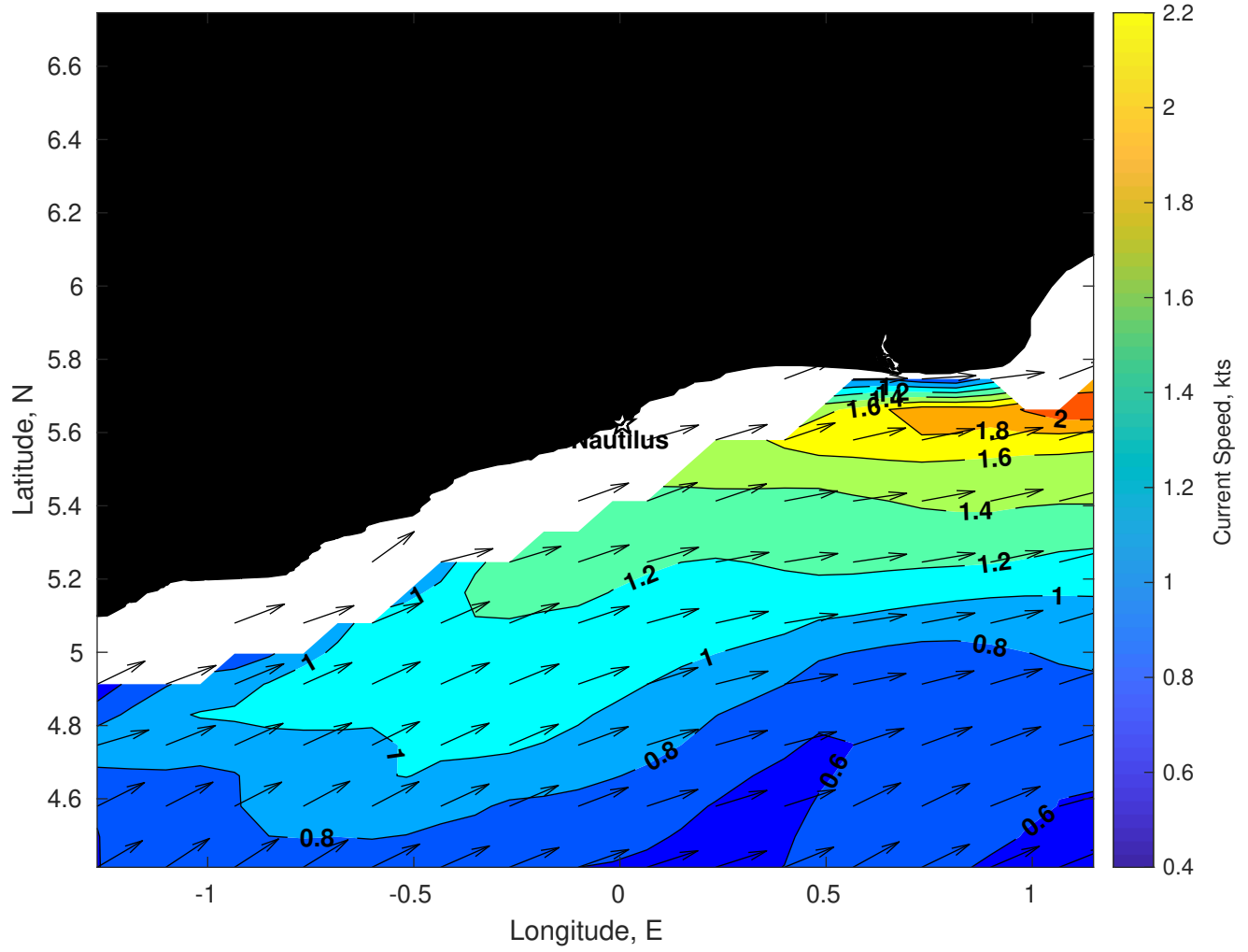
Surface Currents for Nautilus at 27-Mar-2025 00:00:00
