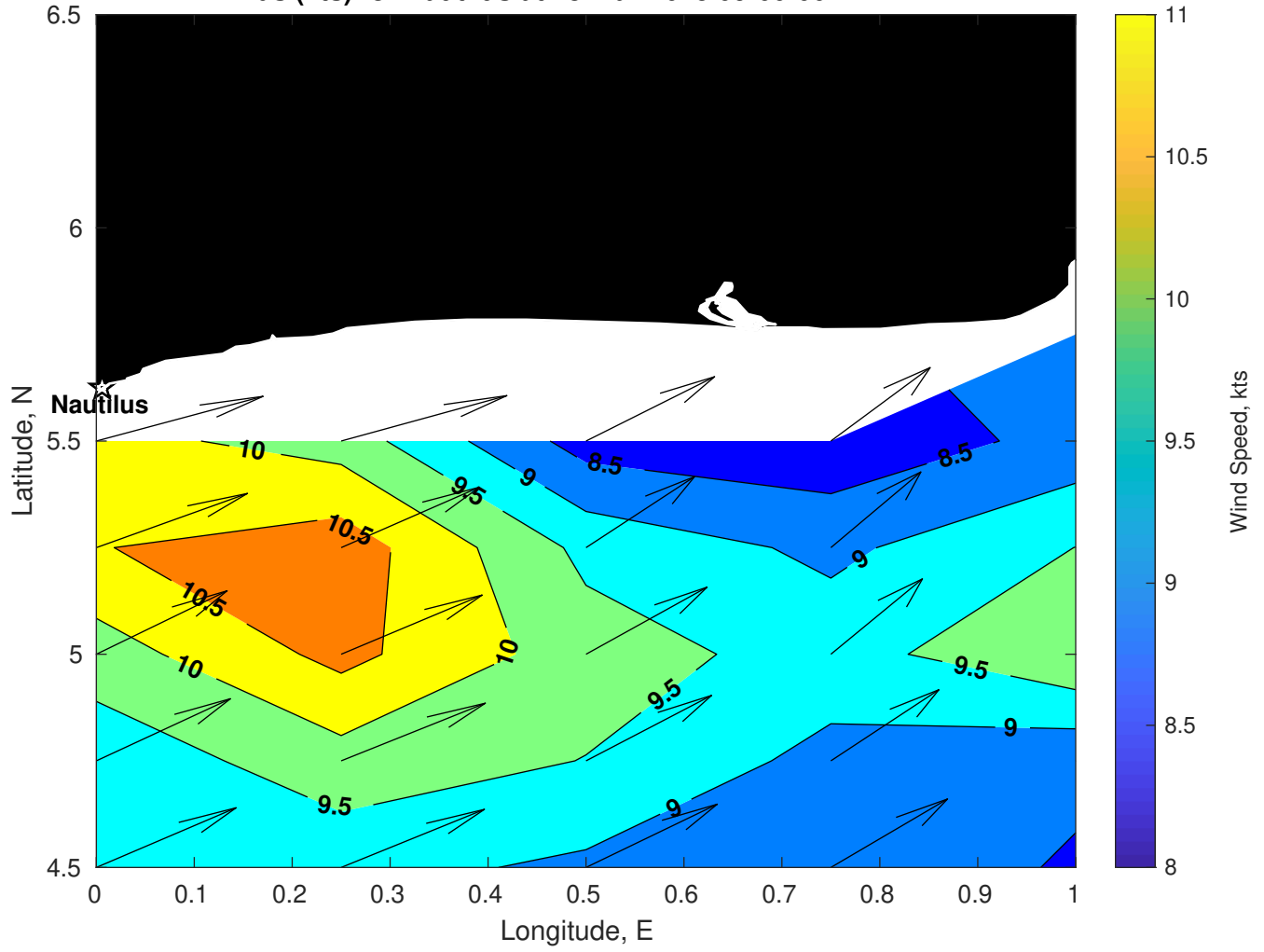
Winds (kts) for Nautilus at 28-Mar-2025 09:00:00
