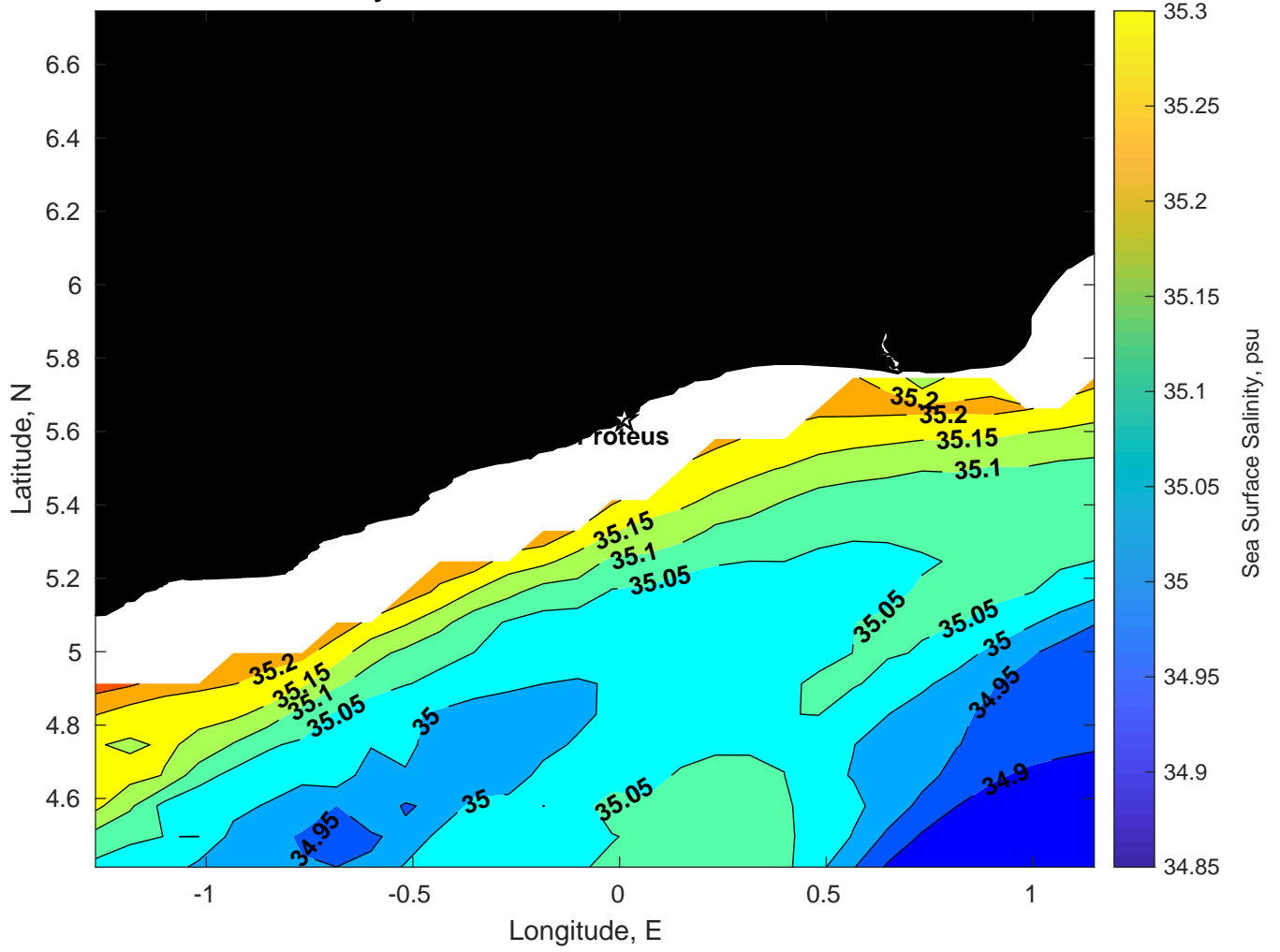
Surface Salinity for Proteus at 27-Mar-2025 00:00:00
