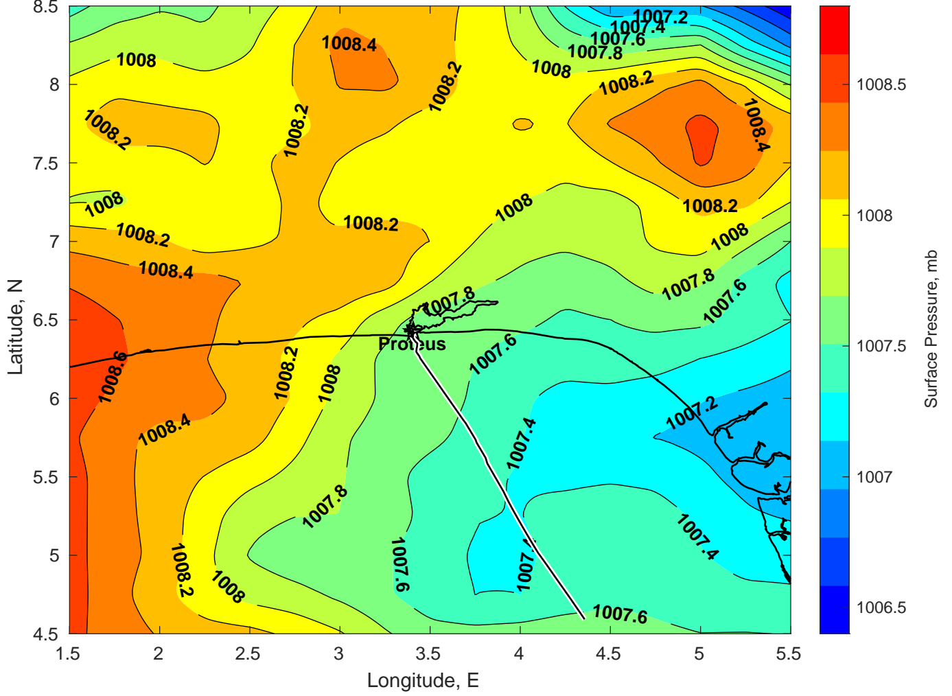
Surface Pressure (mb) for Proteus at 30-Mar-2025 00:00:00
