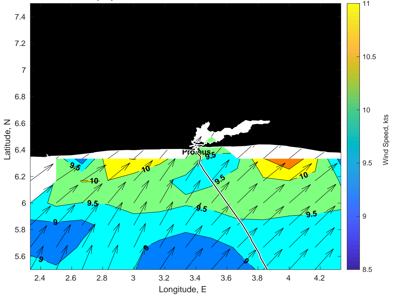
Winds (kts) for Proteus at 28-Mar-2025 09:00:00
