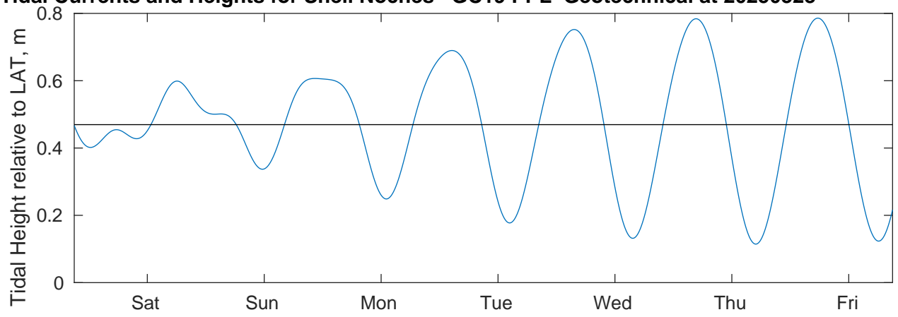
Tidal Currents and Heights for Shell Noches GC19 PPL Geotechnical at 20250328
