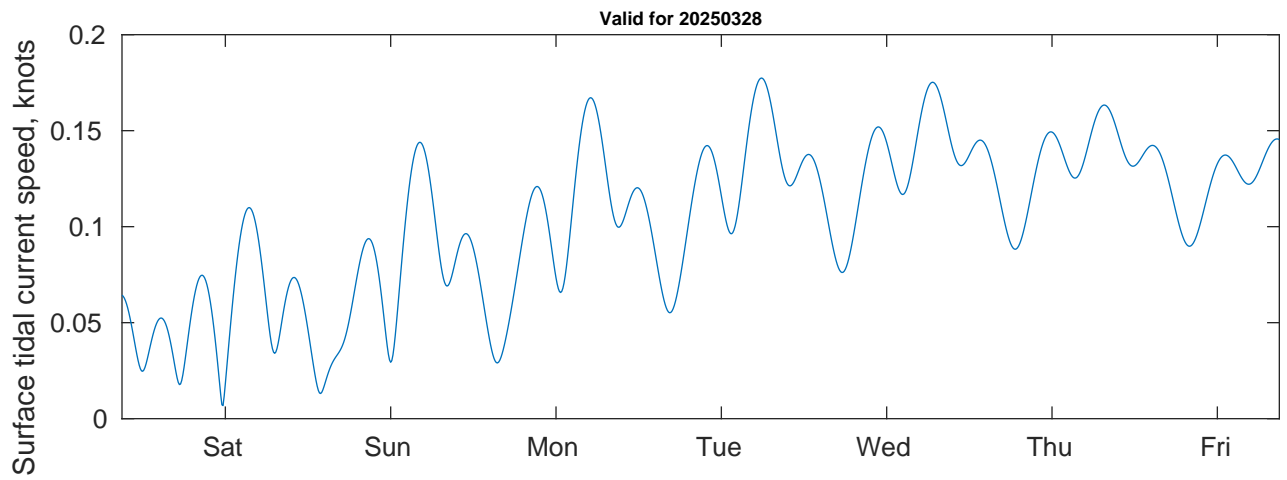
Tidal Currents and Heights for Shell Noches GC19 PPL Geotechnical at 20250328
