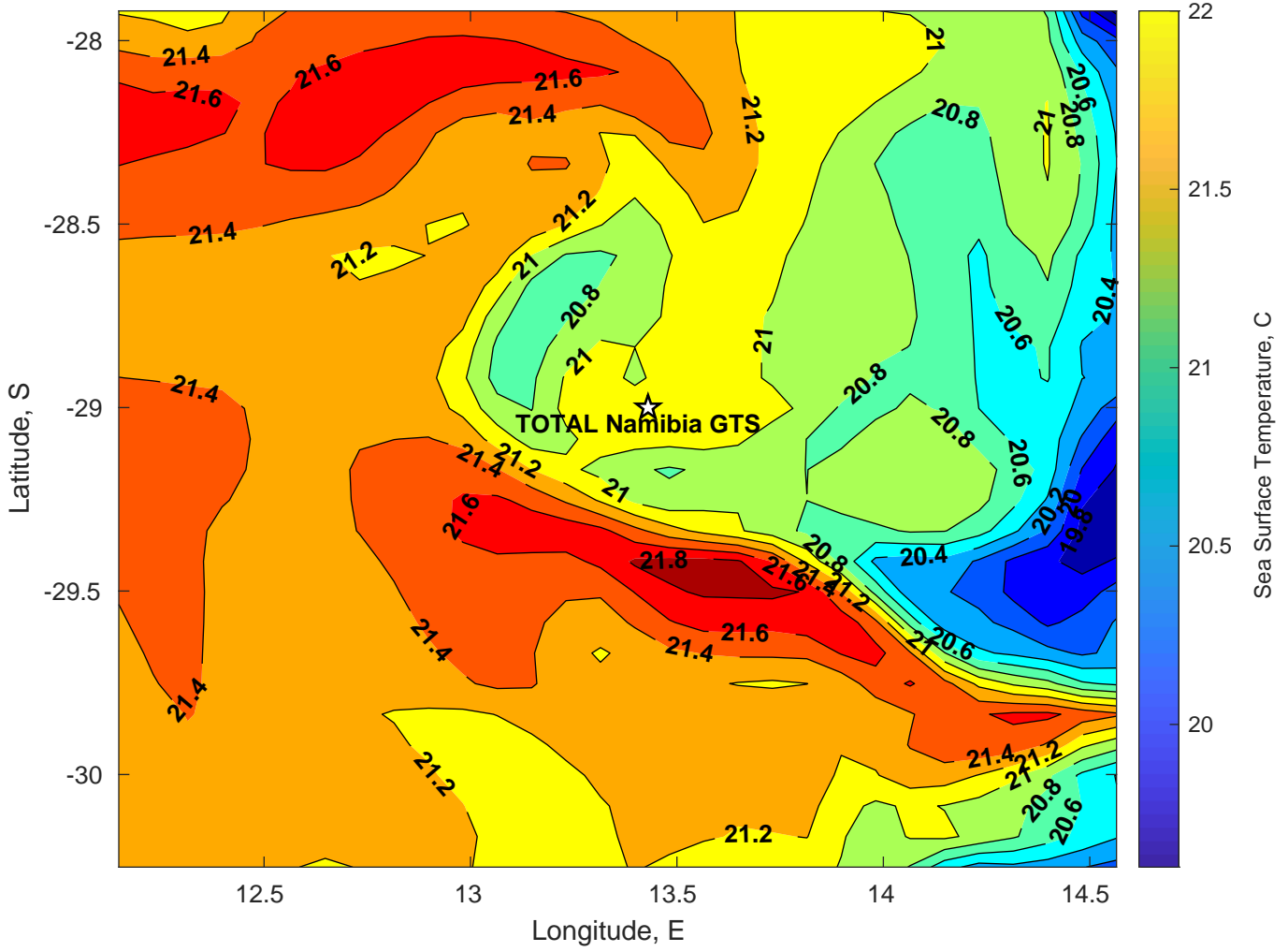
SST for TOTAL Namibia GTS at 27-Mar-2025 00:00:00
