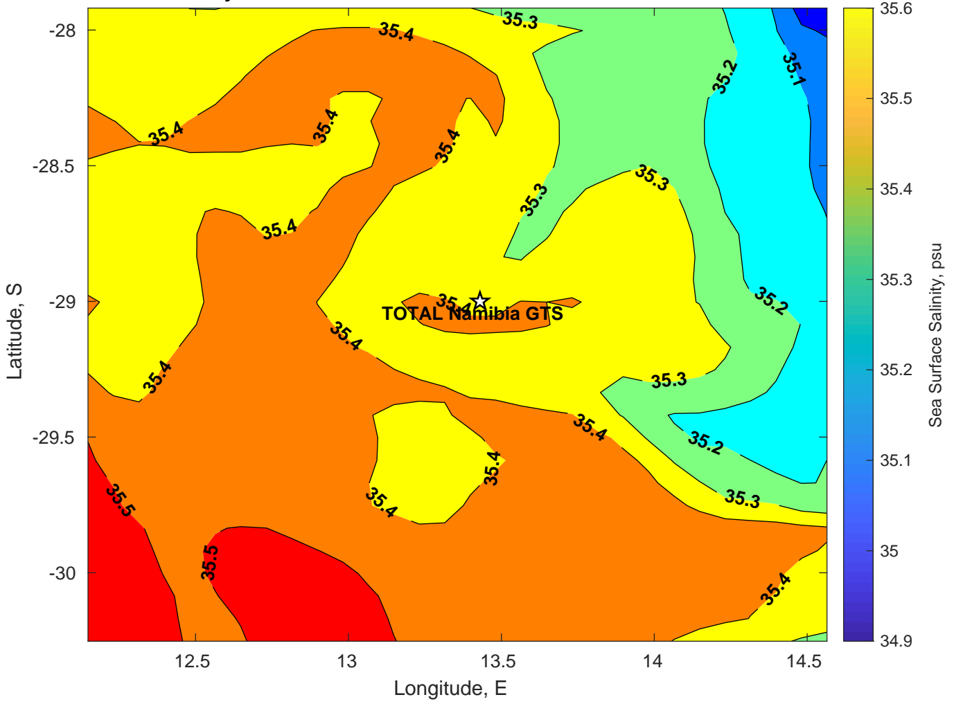
Surface Salinity for TOTAL Namibia GTS at 27-Mar-2025 00:00:00
