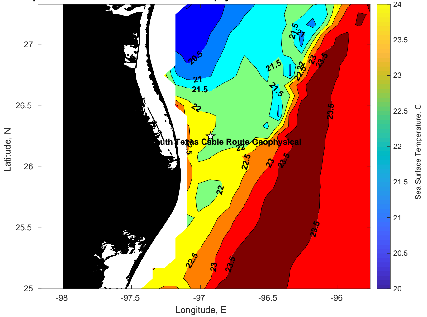
SST for Tampnet P2378 South Texas Cable Route Geophysical at 27-Mar-2025 00:00:00
