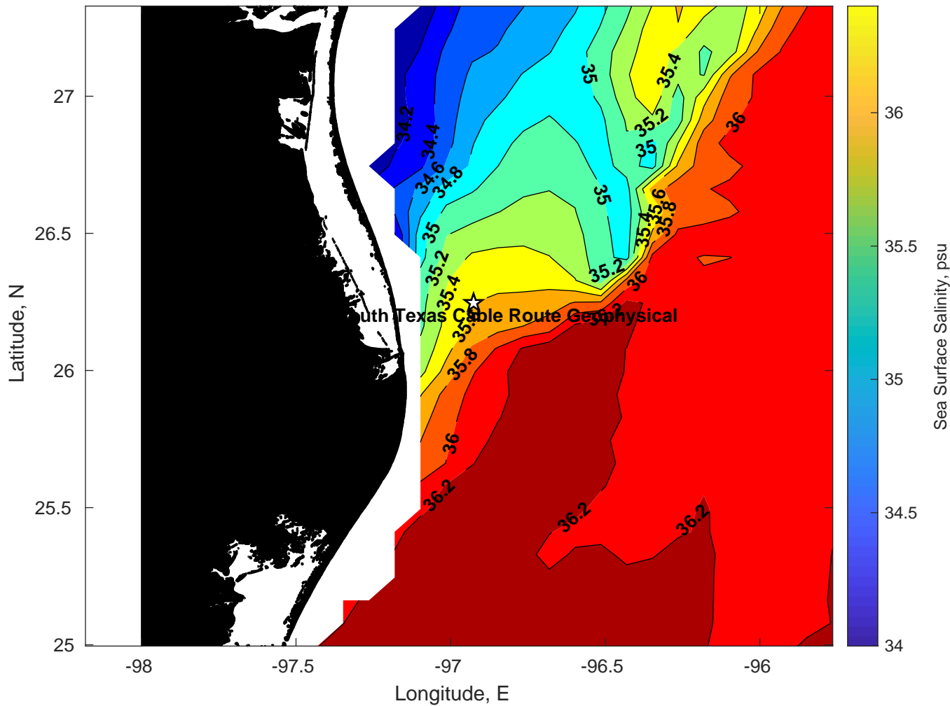
Surface Salinity for Tampnet P2378 South Texas Cable Route Geophysical at 27-Mar-2025 00:00:00
