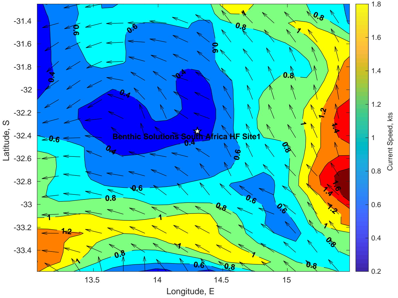
Surface Currents for Benthic Solutions South Africa HF Site1 at 28-Mar-2025 00:00:00
