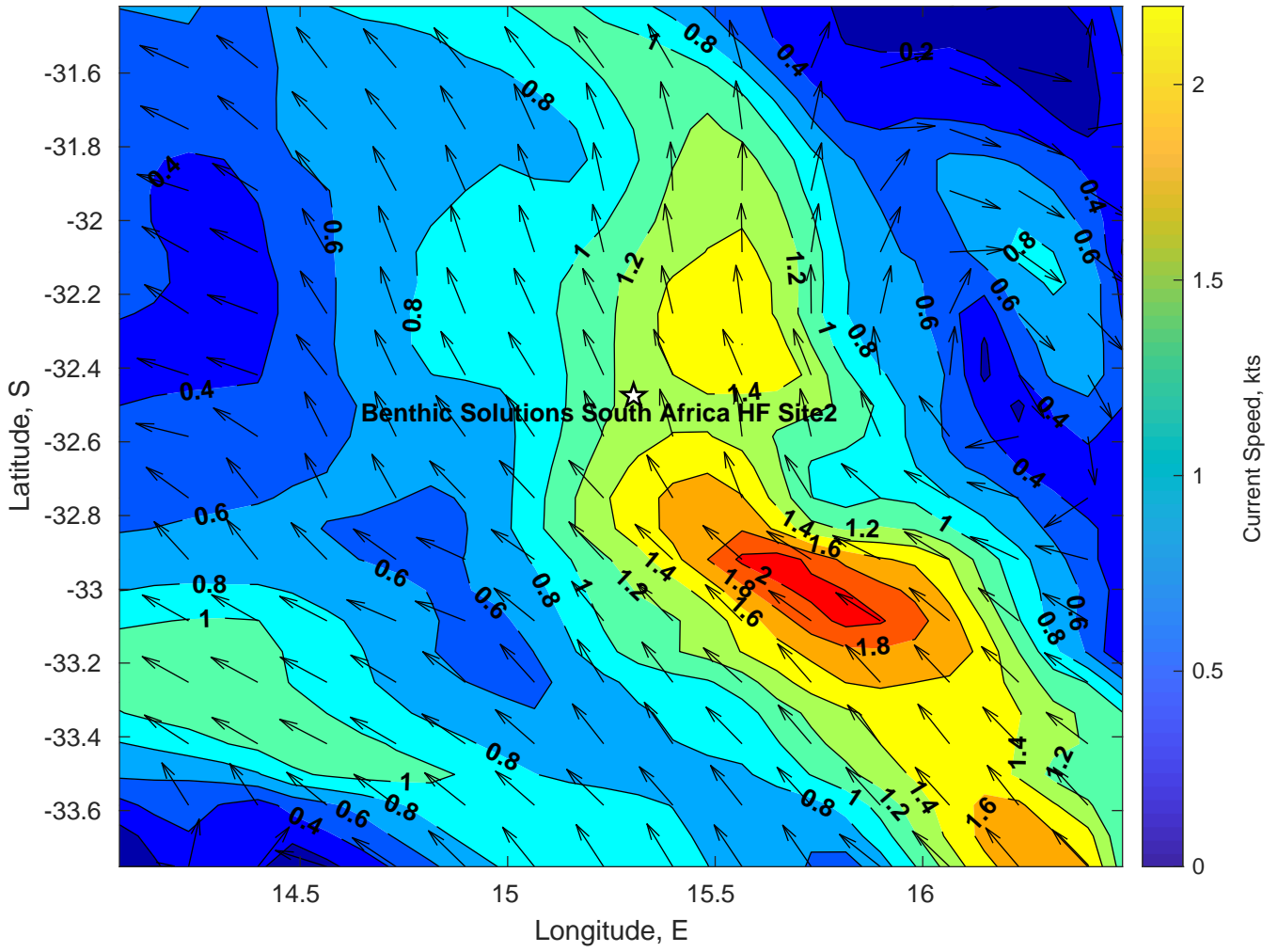
Surface Currents for Benthic Solutions South Africa HF Site2 at 28-Mar-2025 00:00:00
