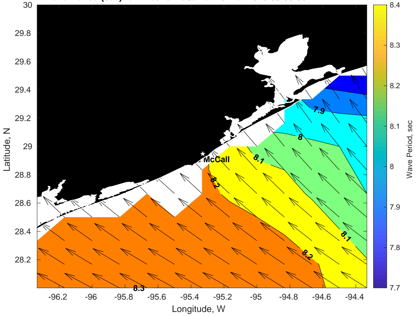
Wave Period (sec) for Brooks McCall at 29-Mar-2025 09:00:00
