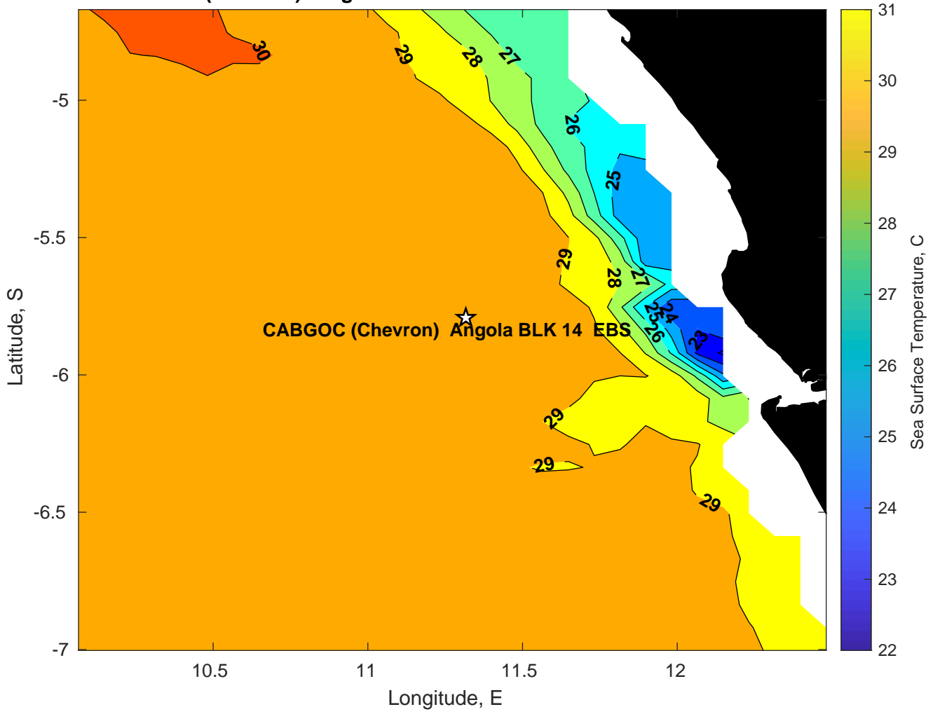
SST for CABGOC (Chevron) Angola BLK 14 EBS at 28-Mar-2025 00:00:00
