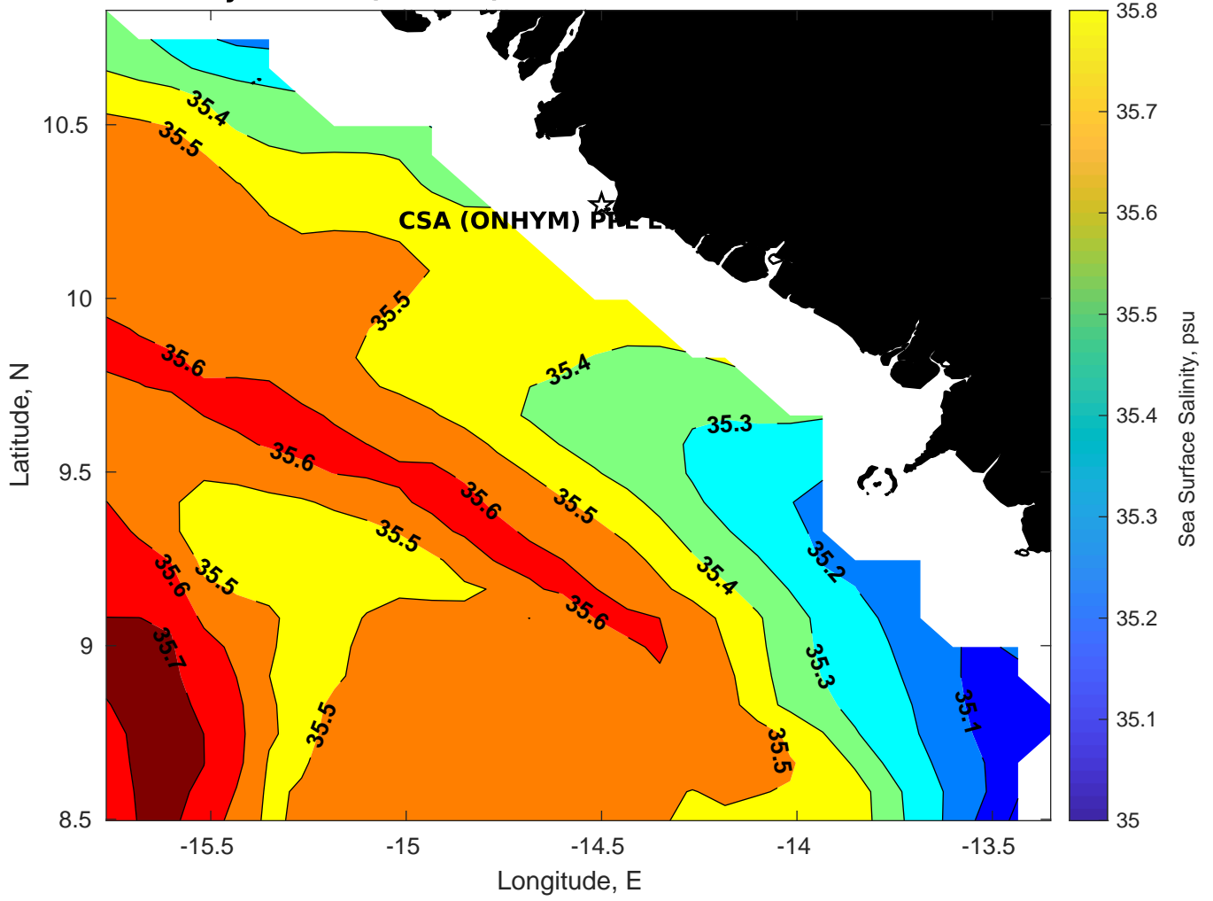
Surface Salinity for CSA (ONHYM) PPL EBS - Guinea at 28-Mar-2025 00:00:00
