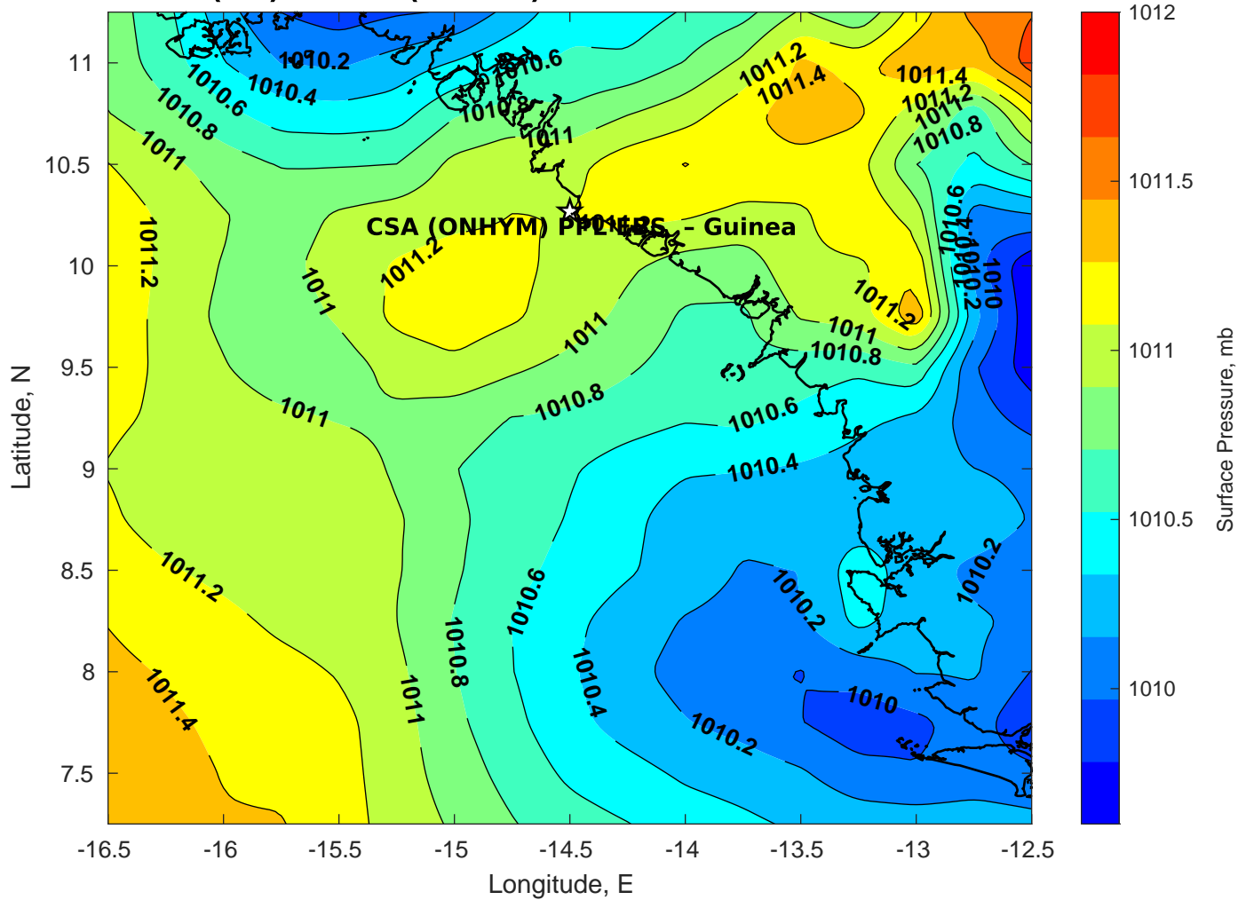
Surface Pressure (mb) for CSA (ONHYM) PPL EBS - Guinea at 30-Mar-2025 00:00:00
