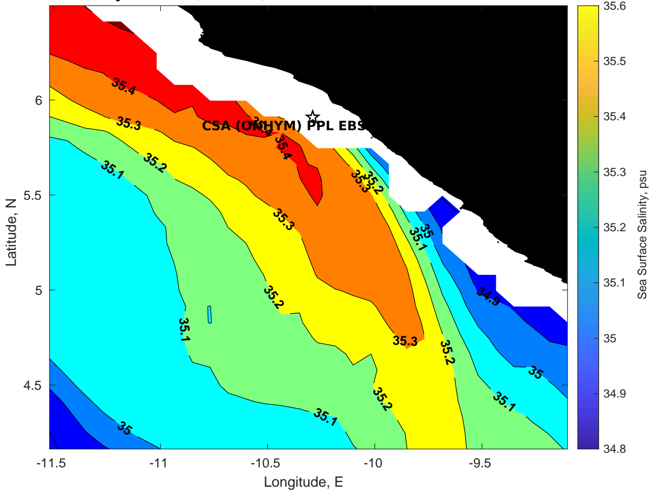
Surface Salinity for CSA (ONHYM) PPL EBS - Liberia at 28-Mar-2025 00:00:00
