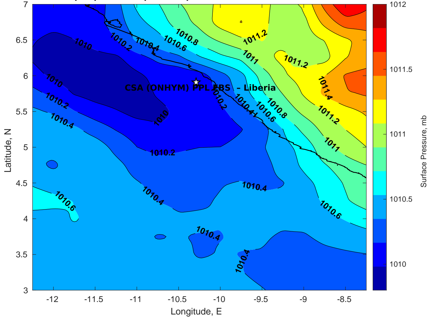
Surface Pressure (mb) for CSA (ONHYM) PPL EBS - Liberia at 31-Mar-2025 00:00:00
