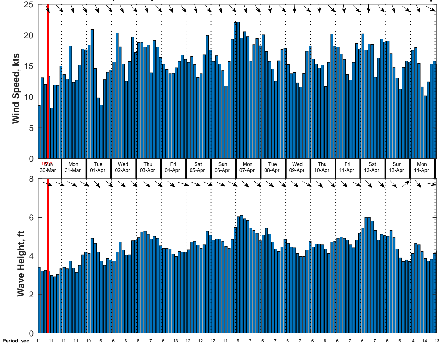
Wind & Wave Forecast for CSA (ONHYM) PPL EBS - Mauritania from 29-Mar-2025 01:00:00 to 14-Apr-2025 01:00:00
