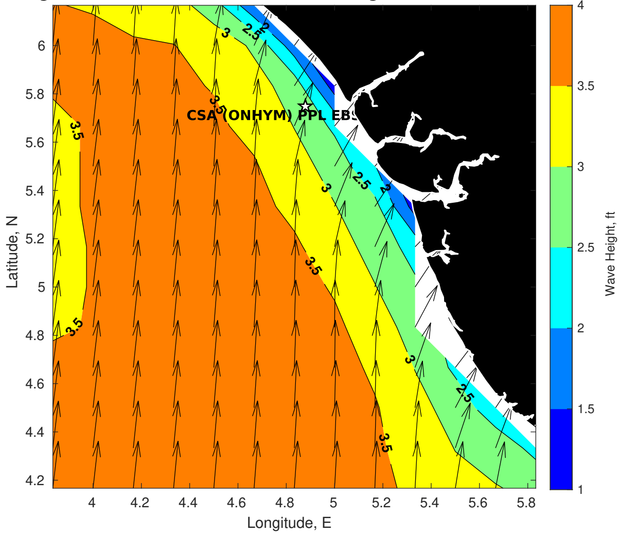
Wave Height (ft) for CSA (ONHYM) PPL EBS - Nigeria at 29-Mar-2025 09:00:00
