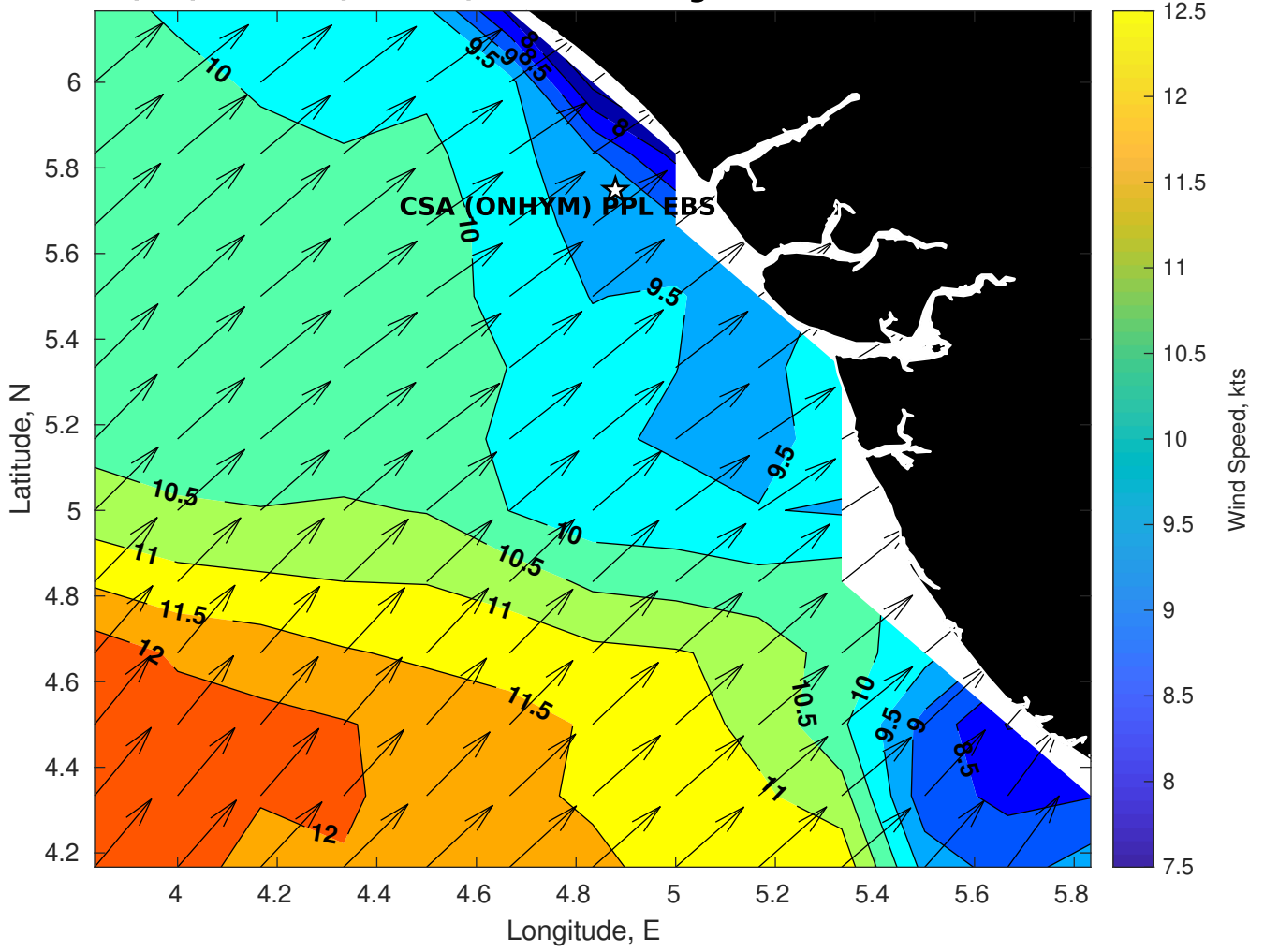
Winds (kts) for CSA (ONHYM) PPL EBS - Nigeria at 29-Mar-2025 09:00:00
