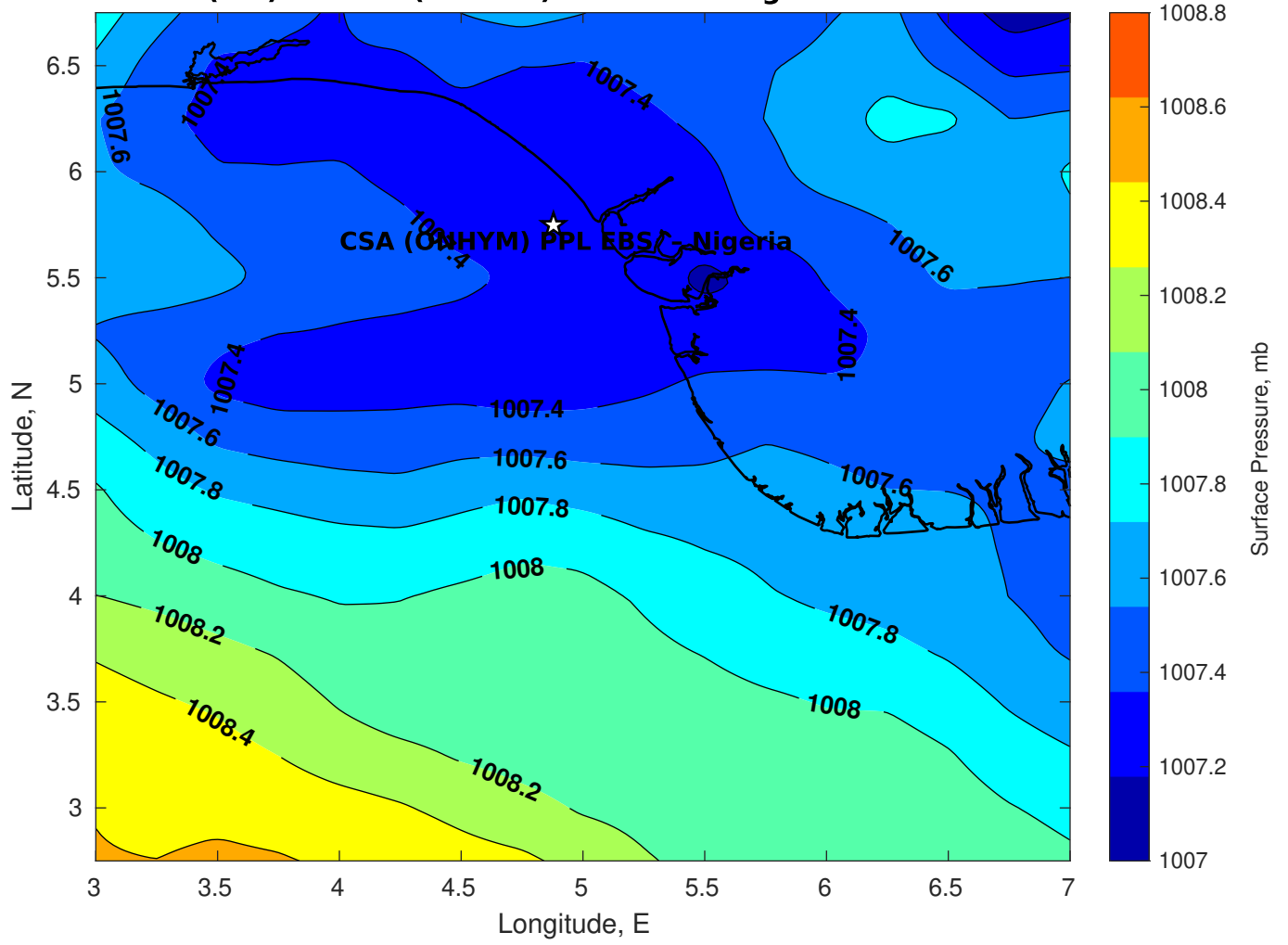
Surface Pressure (mb) for CSA (ONHYM) PPL EBS - Nigeria at 30-Mar-2025 00:00:00
