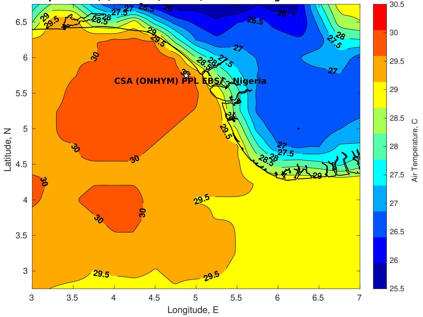
Air Temperature (C) for CSA (ONHYM) PPL EBS - Nigeria at 29-Mar-2025
