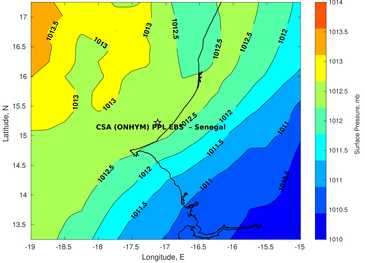
Surface Pressure (mb) for CSA (ONHYM) PPL EBS - Senegal at 29-Mar-2025 00:00:00
