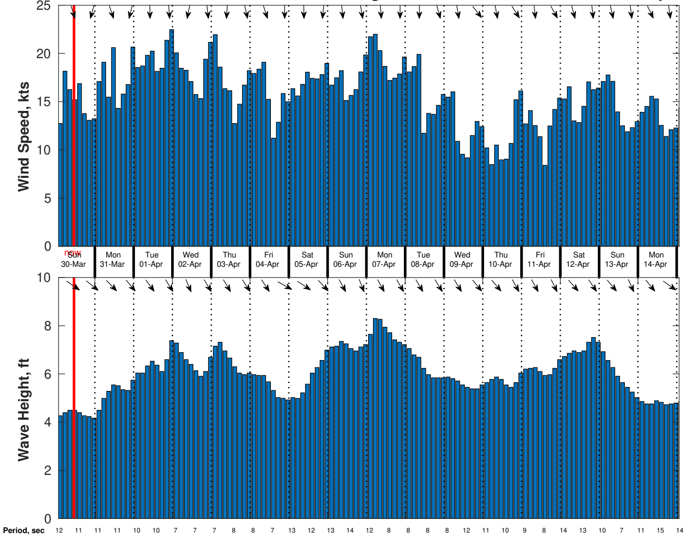
Wind & Wave Forecast for CSA (ONHYM) PPL EBS - Senegal from 29-Mar-2025 01:00:00 to 14-Apr-2025 01:00:00
