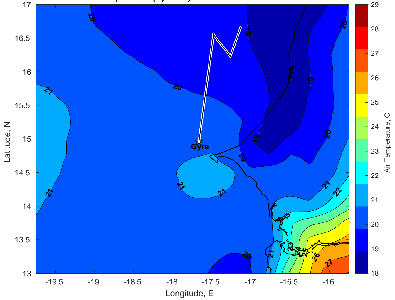
Air Temperature (C) for Gyre at 29-Mar-2025
