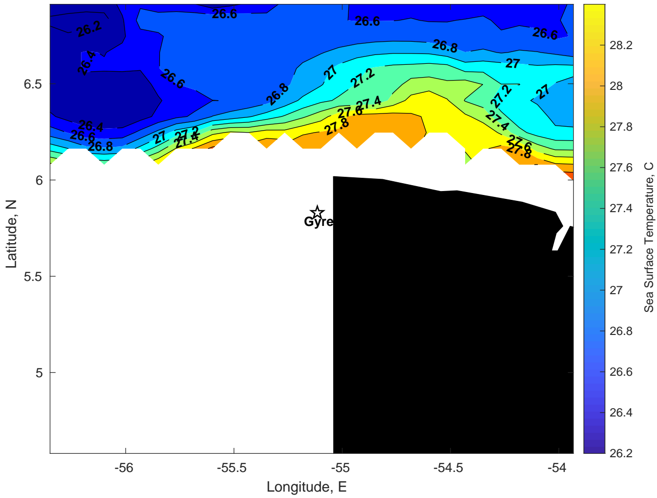
SST for Gyre at 28-Mar-2025 00:00:00
