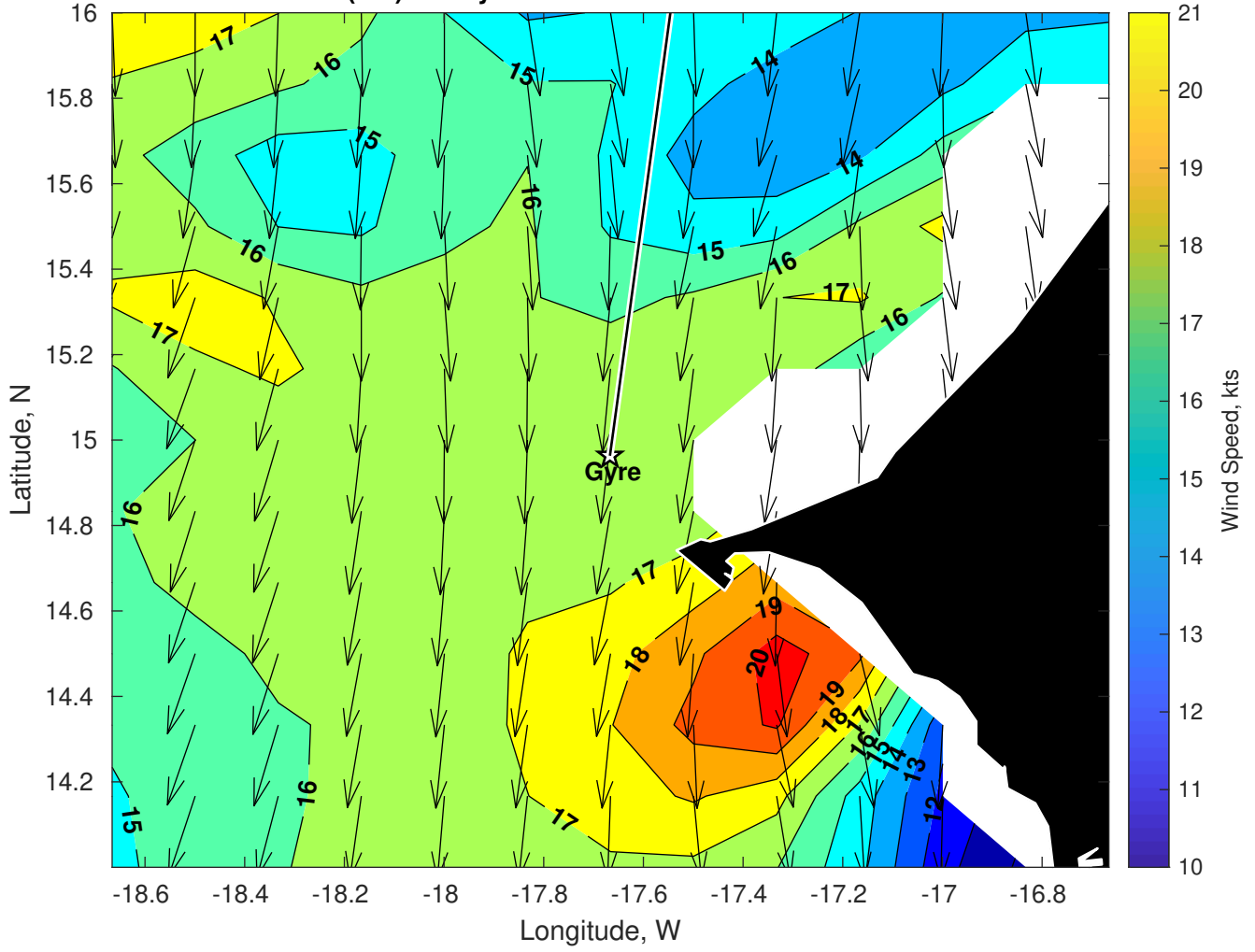
Winds (kts) for Gyre at 29-Mar-2025 09:00:00
