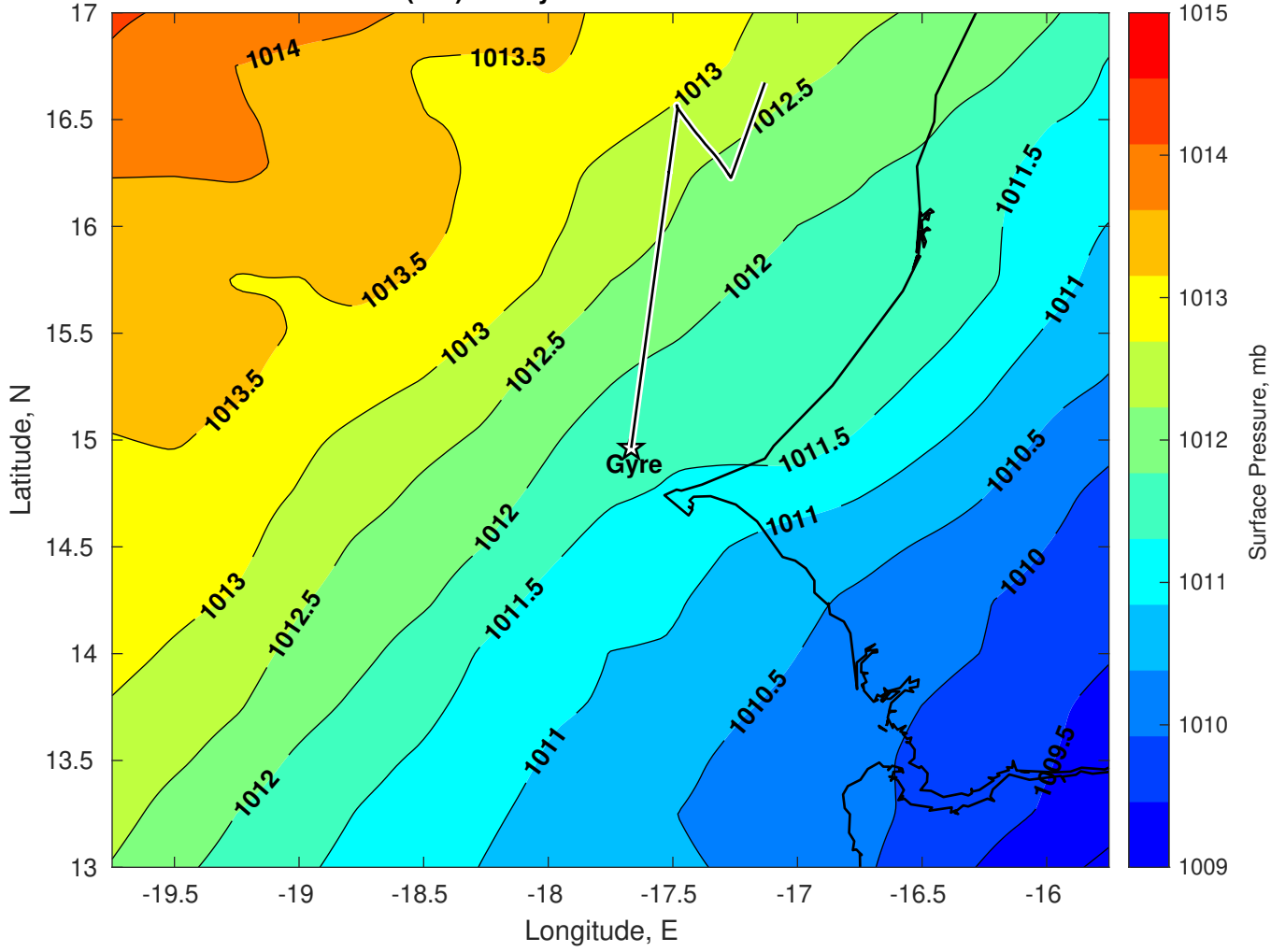
Surface Pressure (mb) for Gyre at 31-Mar-2025 00:00:00
