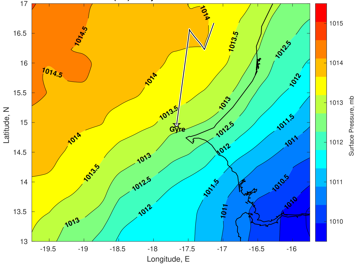
Surface Pressure (mb) for Gyre at 30-Mar-2025 00:00:00
