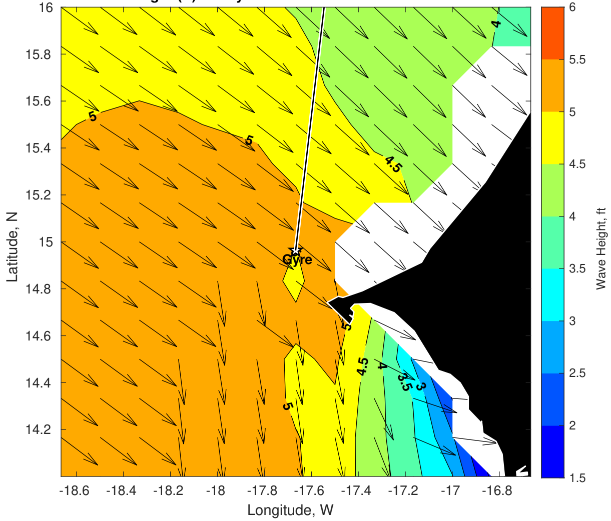
Wave Height (ft) for Gyre at 29-Mar-2025 09:00:00
