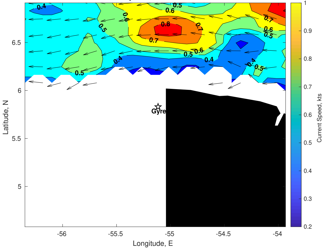
Surface Currents for Gyre at 28-Mar-2025 00:00:00
