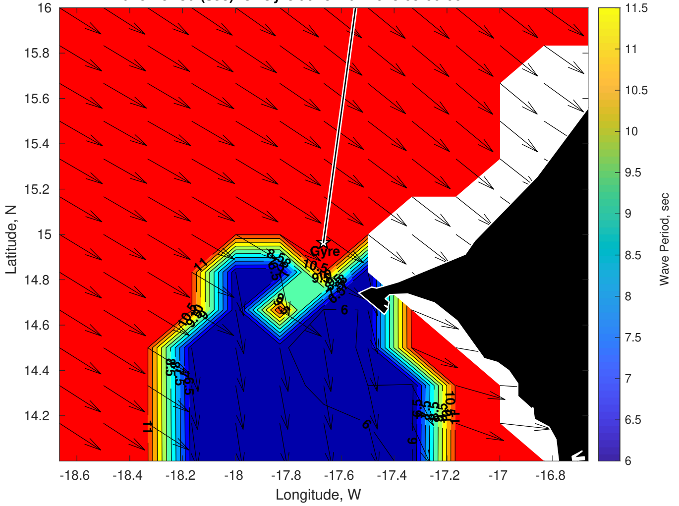
Wave Period (sec) for Gyre at 29-Mar-2025 09:00:00
